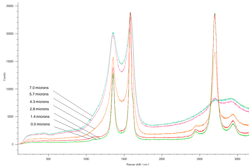
Figure 5b. Coated Fiber with CsI Coating at 200,000 shots
