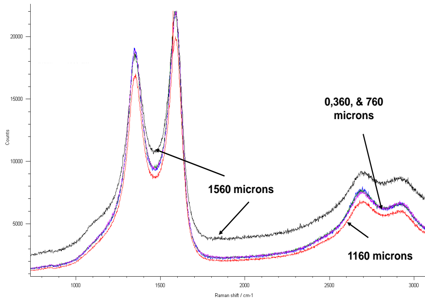
Figure 5a. Uncoated Fibers with no CsI Coating
