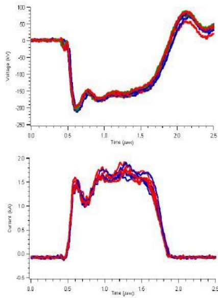
Figure 2: Current and Voltage Traces During Standard Operation of the Experiment. The ripple on current and voltage traces stems from mismatches in the PFN and Diode, and occurs even with a resistive load.
