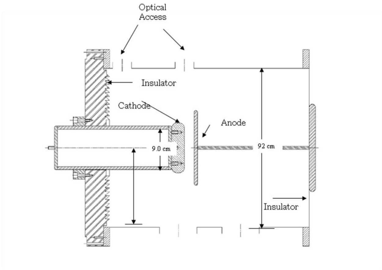
Figure 1: Experimental Schematic
