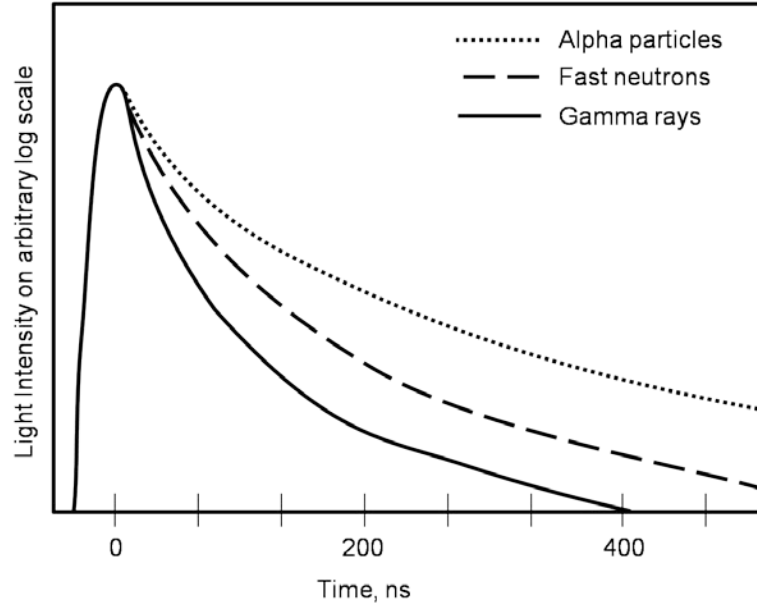
Figure 29: Decay Components for PSD. Alpha particles are the heaviest particles shown and the pulses that correspond to alpha particles have the longest decay components. Pulses that arise from gamma ray interactions have the shortest decay time. The heavier particles have a longer decay time for the same light output than the lighter particles [8].
