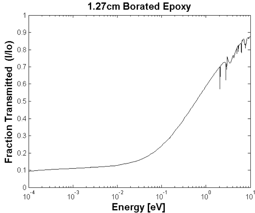
Figure 8: Fraction Transmitted for 1.27 cm Borated Epoxy. The fraction transmitted was calculated at each energy for the thickness of the mask using equation (1.3). Note that the fraction transmitted does not drop as low as it does for cadmium, but it also attenuates more at higher energies. It exhibits some resonance behavior.
