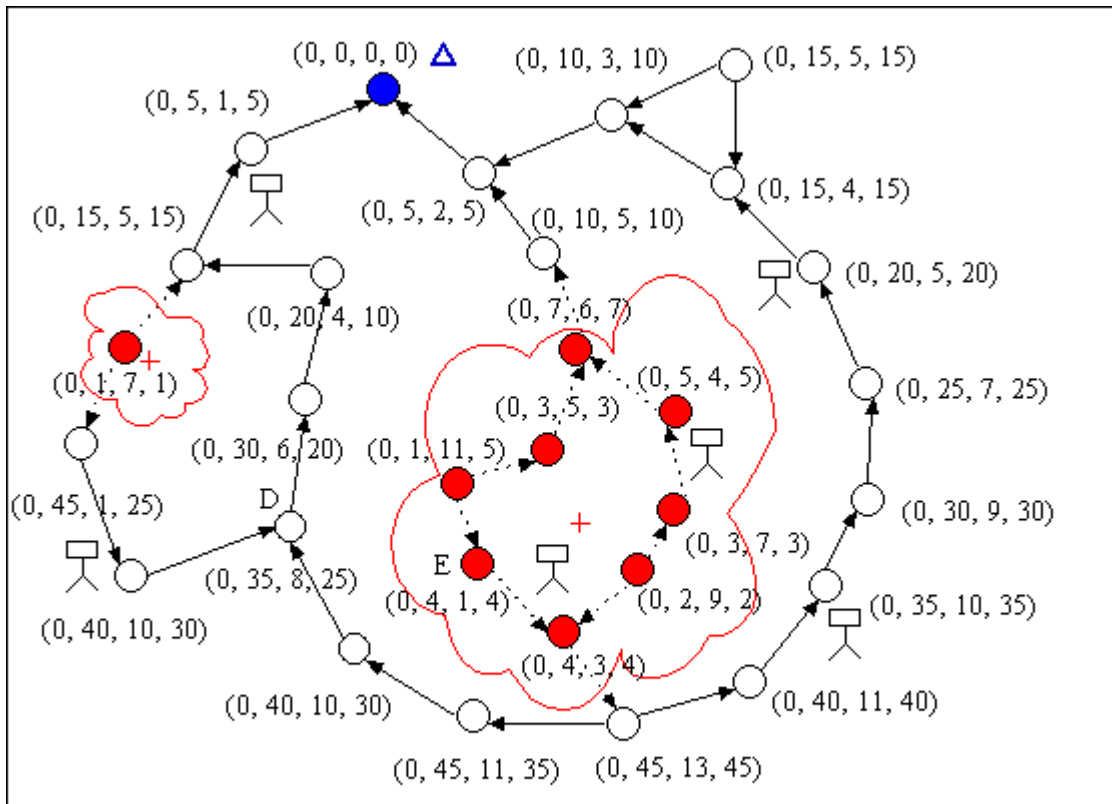
Figure 4: A sample scenario to demonstrate a directed navigation graph constructed by our distributed path planning algorithms.
