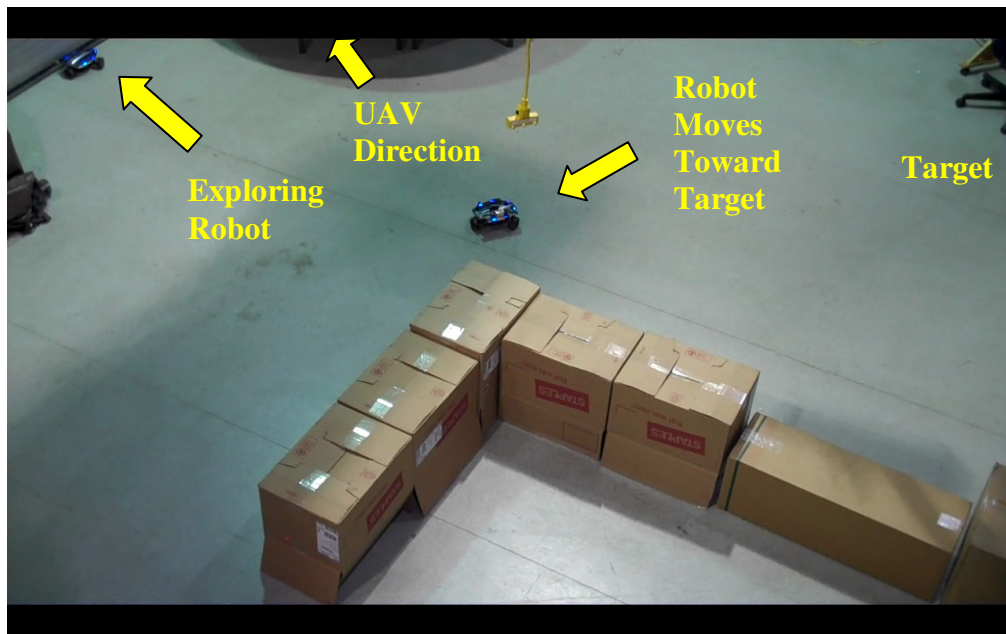
Figure 12. The UAV has identified the target, and the team of UGVs begins their mission. One of the ground vehicles begins to move to the target, while the rest explore the environment. As the target moves, the UAV provides updates to the UGVs within the building. (The UAV is outside of the frame toward the upper left.)
