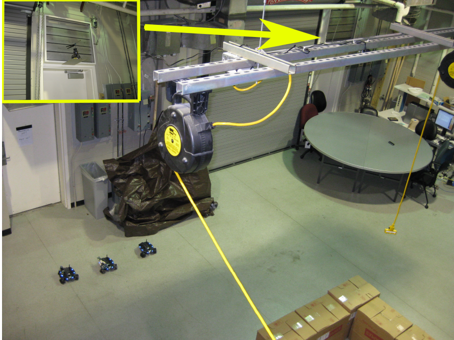
Figure 2. Environment for the experiment, with the three ground robots in place and the aerial vehicle perched.
