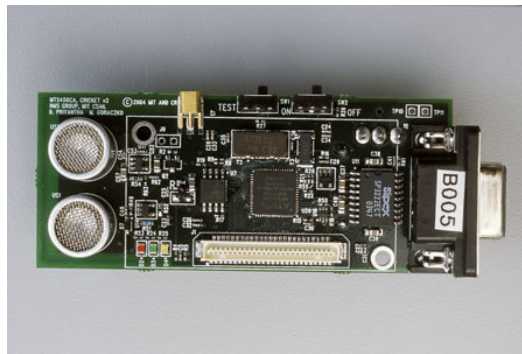
Figure 10. A Cricket indoor localization developed by MIT and manufactured by Crossbow. Each listener mote determines its position based upon the position of several beacon motes.
