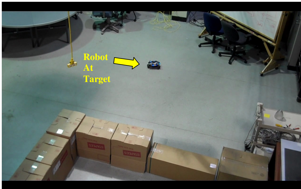
Figure 13. The robot arrives at the target. After encountering the target, all of the robots further explore the environment in order to ensure the target may be continuously tracked in addition to generating additional intelligence in the form of a map.
