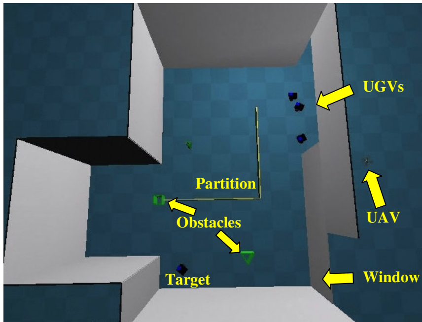
Figure 6. Initial scenario configuration within the MissionLab/Gazebo simulation environment. The team of UGVs stand ready at the entrance of the building while the UAV begins moving towards the window for an interior view.
