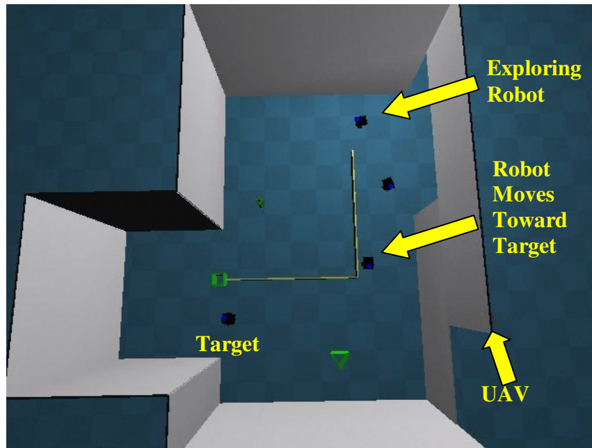
Figure 7. The UAV has positioned itself at the window and has identified the target. The team of UGVs enter the building in a loose formation. One of the ground vehicles begins to move to the target, while the rest spread out and explore the environment. As the target moves, the UAV provides updates to the UGVs within the building. (The UAV is partially obscured by the wall due to the camera angle of the simulation.)
