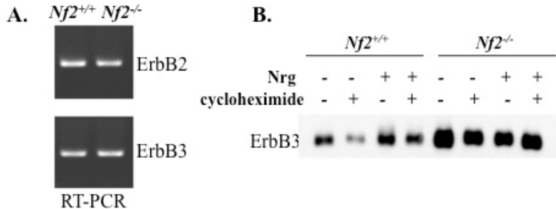
Figure 14: Merlin controls ErbB3 stability. A. The levels of ErbB2 and ErbB3 mRNA were similar in wild-type and Nf2 -/- SCs; however, the levels of ErbB3 protein were higher in the Nf2 -/- SCs. B. Cyclohexamide treatment yielded a further decrease in ErbB3 levels in the wild-type SCs in the presence and absence of Nrg. In contrast, cyclohexamide had little effect on the high levels of ErbB3 in Nf2 -/- SCs.
