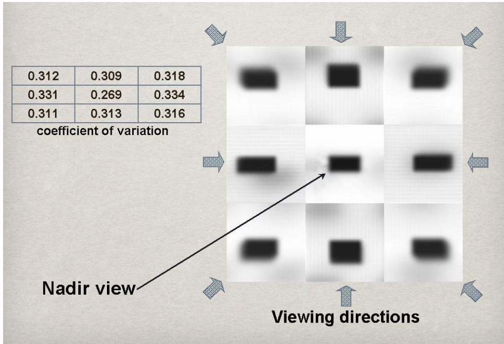
Figure 3. Example of the effects of viewing angle on model images of a black vehicle of 2m vertical thickness at 1.5 m depth over a bright bottom at 10m depth. CV values for each of nine views are shown in the matrix box: nadir (center) and eight azimuthal views every 45^\circ .
