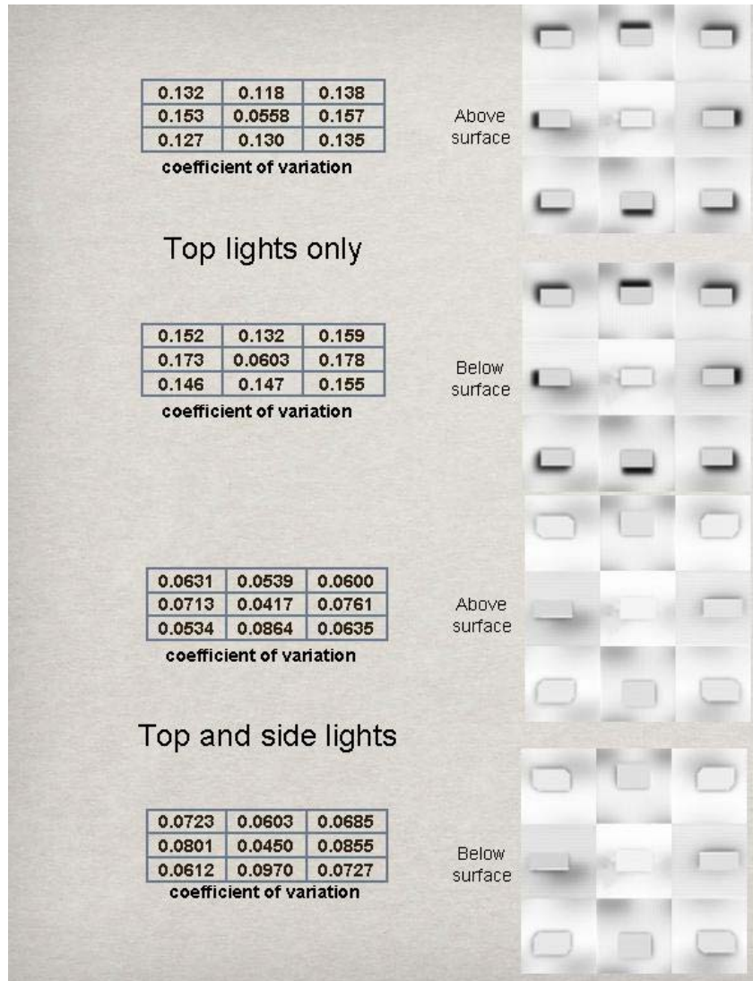
Figure 4. Contrast results with arrays of top lights and top plus side lights.
