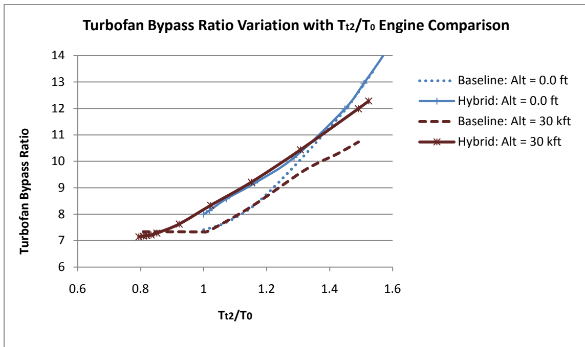
Figure 4.14 Turbopan bypass ratio variation with T_{t2}/T_0 comparison of the baseline and hybrid engines at SLS and cruise (maximum thrust)
