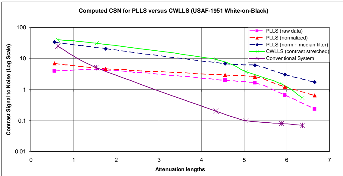
Figure 5: Contrast Signal Noise Ratio versus number of attenuation lengths for gated-PLLS, CWLLS and conventional camera and light.
