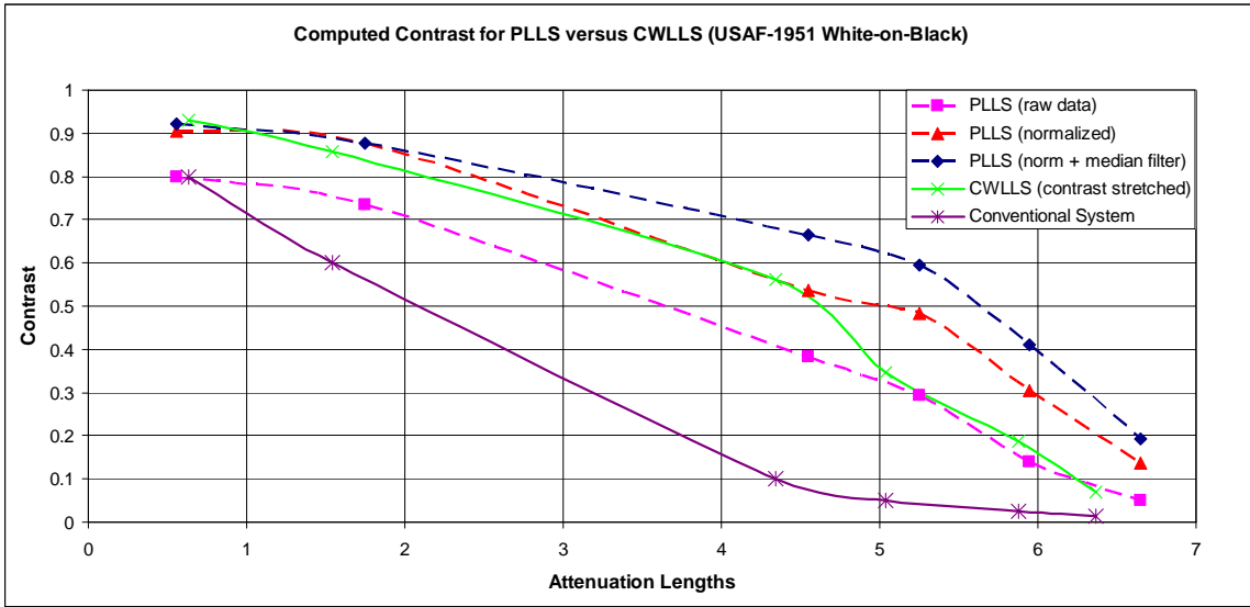
Figure 4: Contrast versus number of attenuation lengths for gated-PLLS, CWLLS and conventional camera and light.
