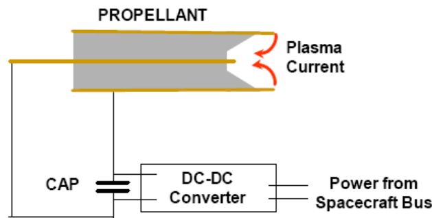
Figure 2: Two-electrode micro-PPT 4
