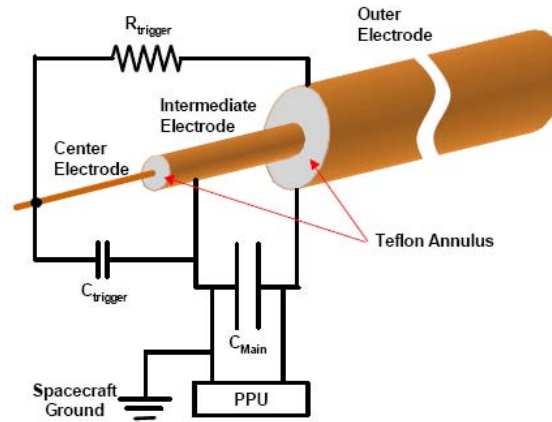
Figure 3: Three-electrode micro-PPT 4
