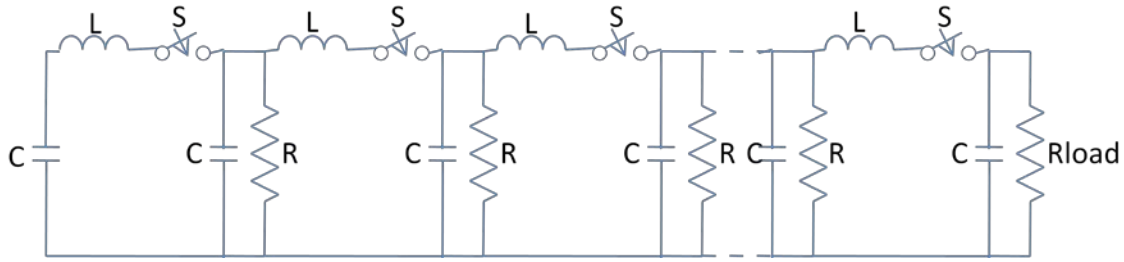
Figure 5: Dr. Mesyats more efficient voltage multiplier 5
