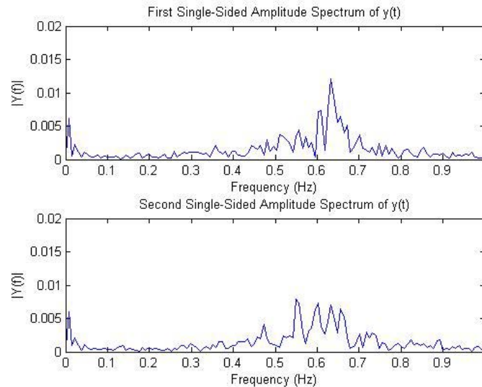
Figure 61 FFT Response for two 50 mHz test runs
