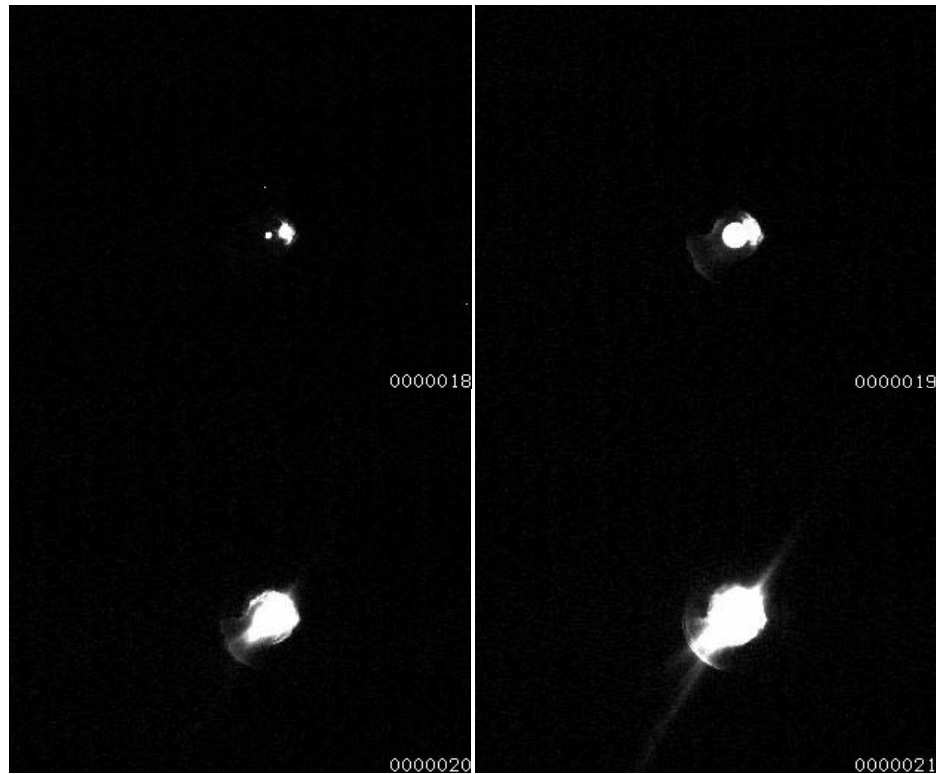
Figure 69 Spark Formation on Mass Collection Thruster
