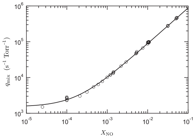
FIG. 4. Measured quenching rate coefficients for NO/N 2 mixtures at 294 K (circles). Equation (3) was fitted to the data (solid curve) to yield best-fit values of q_{\text{NO}} = 8.77 \times 10^6 \text{ s}^{-1} \text{ Torr}^{-1} and q_{\text{N}_2} = 1.5 \times 10^3 \text{ s}^{-1} \text{ Torr}^{-1} .
