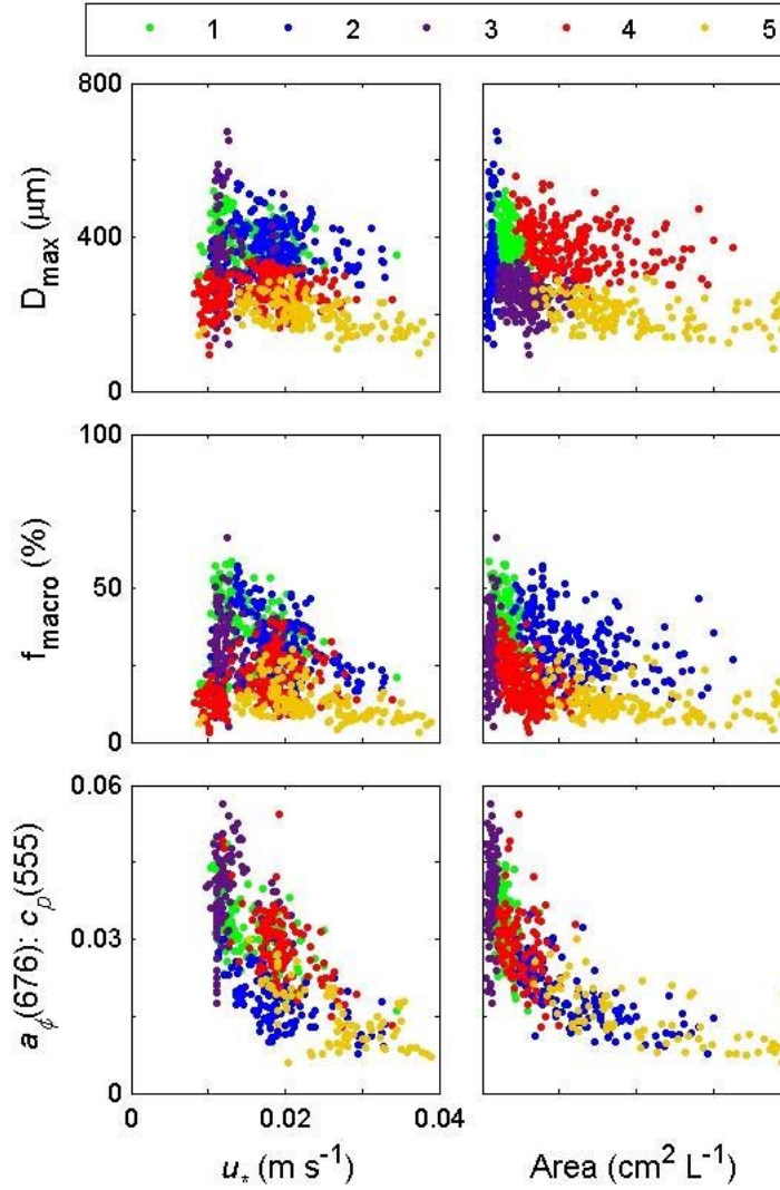
Figure 1. Maximum floc size ( D_{\max} ) (top row), floc fraction ( f_{\text{macro}} ) (middle row), and the ratio a_{\phi}(676) c_p(555)^{-1} (bottom row) versus combined wave-current turbulent shear velocity ( u_* ) (left column) and area concentration in suspension (right column). The ratio a_{\phi}(676) c_p(555)^{-1} is a relative measure of the amount of pigmented particles to total particles in suspension. Different colors denote the 5 entropy groups, which contain statistically similar size distributions. Plots of maximum floc size versus shear velocity and suspended area are wedge-shaped, with a large spread of floc sizes at small shear velocities and suspended areas. The distributions of values of maximum floc size taper to small spreads at larger shear velocities and suspended area concentrations. The taper arises from a reduction in the upper limit of observed sizes. The largest observed floc sizes are about 600 micrometers. At high stresses and areas, this upper limit decreases to about 200 micrometers. This same pattern holds for floc fraction. At low shear velocities and suspended areas, floc fraction ranges from 0.1 to 0.75. At high shear velocities and suspended areas, floc fractions are all around 0.1. The optical ratio shows more of a hyperbolic distribution, decreasing from high values of around 0.06 at low shear velocities and suspended areas to low values of around 0.01 for higher shear velocities and areas.
