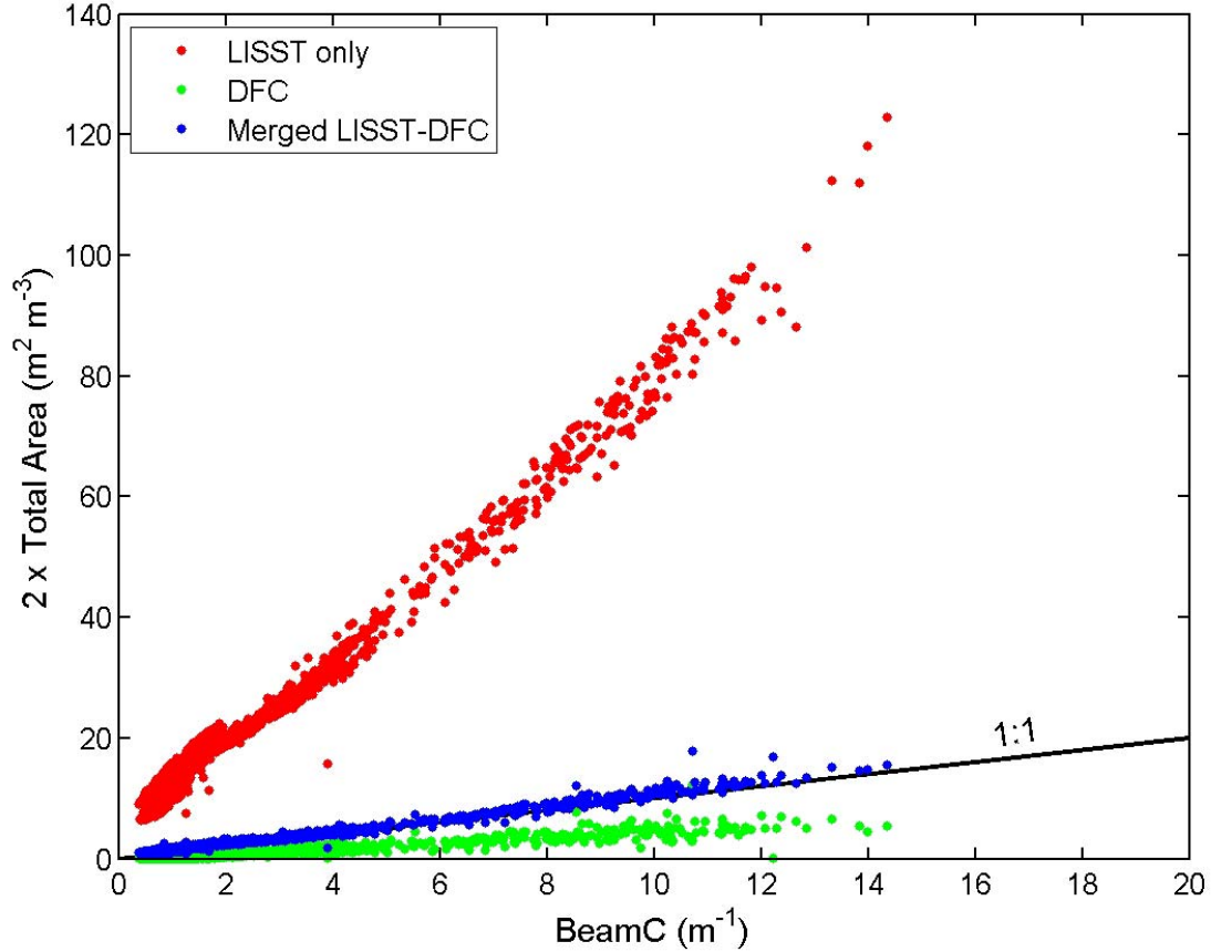
Figure 4. Plot of 2 times the suspended particle projected area measured 3 ways on the y axis versus the attenuation coefficient on the x axis. Also shown is a 1:1 line. Theoretically, if the particles are much larger than the wavelength of light, then the data should plot along the 1:1 line. When suspended area is estimated from the DFC, the data plot below the 1:1 line, indicating that the DFC alone underestimates the total suspended area concentration. This result arises because the camera does not resolve particles smaller than 60 \mu\text{m} . When suspended area is estimated from the LISST, which resolves particles between 1.25 and 250 \mu\text{m} , the data plot well above the 1:1 line. In fact, a regression through the data (not shown) has a slope of approximately 10:1, indicating that the LISST is over-estimating suspended area concentration by a factor of 10. The causes of this over-estimation are under investigation. Finally, the data fall close to a 1:1 line if suspended area is estimated from merged size distributions, which are calculated by correcting the LISST concentrations so that they match the DFC concentrations in the region of overlap. This result suggests that the DFC produces more accurate estimates of suspended area concentration.
