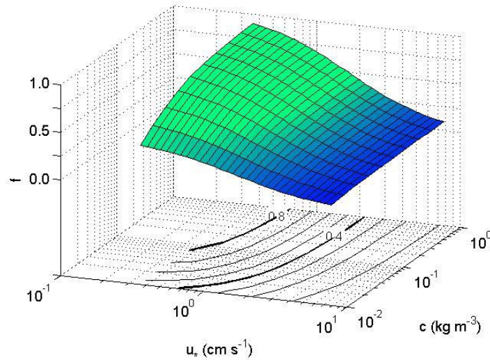
Figure 3. Predicted response of equilibrium floc fraction to changes in shear velocity and sediment concentration. The 3-D shaded surface shows that floc fraction responds primarily to shear velocity when sediment concentration is large. At low sediment concentrations, floc fraction is reduced. Contours of floc fraction below the shaded surface portray these relationships in shear velocity/concentration space. When shear velocity is below 1 \text{ cm s}^{-1} , floc fraction ranges from 0.4 at low concentration to 0.8 at high concentration. As shear velocity increases to 10 \text{ cm s}^{-1} , floc fraction is near zero for all sediment concentrations.
