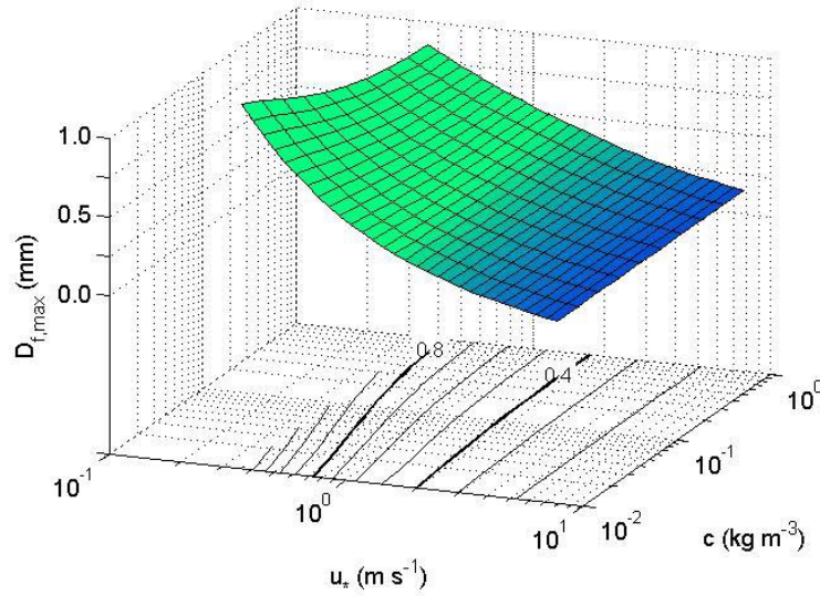
Figure 2. Predicted response of equilibrium maximum floc size to changes in shear velocity and sediment concentration. The 3-D shaded surface shows that floc size responds primarily to shear velocity and has little dependence on sediment concentration. Contours of floc size below the shaded surface plot floc size in shear velocity/concentration space. When shear velocity is below 1 \text{ cm s}^{-1} , floc size approaches 1 mm with the model inputs used here. As shear velocity increases to 10 \text{ cm s}^{-1} , floc size decreases to several hundred micrometers. At these higher shear velocities, floc size does not depend on sediment concentration.
