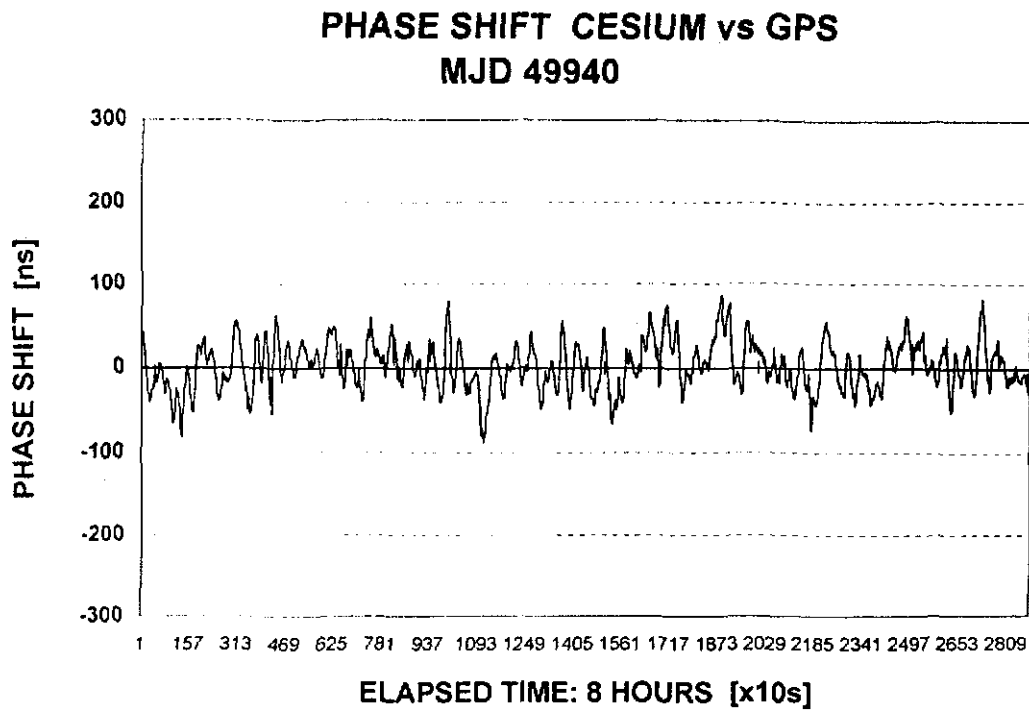
Figure 3. Typical standard frequency signal from GPS (elapsed time: 8 hours).
