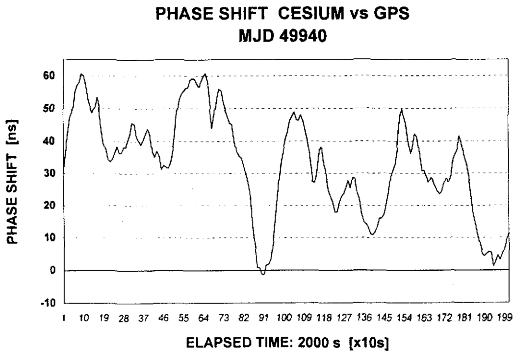
Figure 4. Typical standard frequency signal from GPS (elapsed time: 2,000 s).
