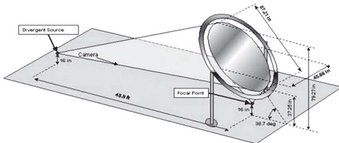
Fig. 12. Test apparatus setup.
