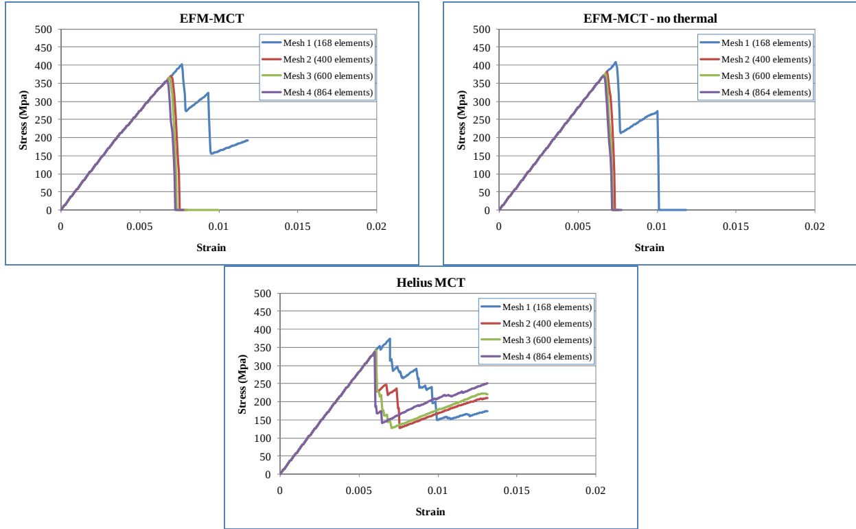
Figure 3 Stress-strain curves
