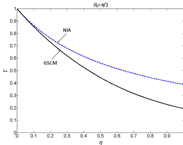
Fig. 3. The calculated \mu^* = C^*_{44} = C^*_{55} for an isotropic solid with randomly oriented cracks.
