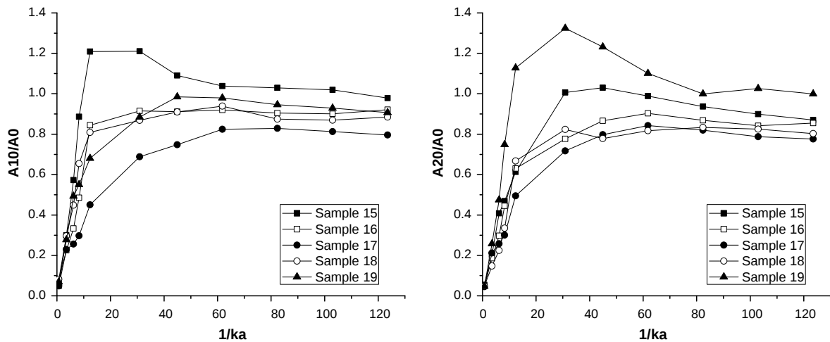
Fig. 16. Output signal strength v.s. 1/ka for tensile waves in the models with \theta_0 = 0^\circ . The crack length 2a is evenly distributed between 0.6 and 1.4, with average of 1.0. Left figure: The normalized peak averaged stress measured at distance equal to 10. Right figure: The normalized peak averaged stress measured at distance equal to 20.
