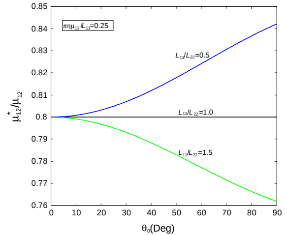
Fig. 2 The variations of \mu_{12}^* of a cracked orthotropic elastic material as a function of \theta_0 by using Eq. 15 for three different values of L_{11}/L_{22} = 0.5, 1.0, 1.5 with \pi \eta \mu_{12}/L_{11} = 0.25
