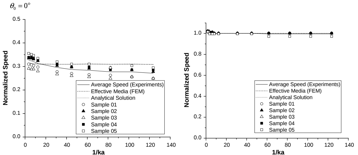
Fig. 8. Normalized wave speed vs. 1/ka for \theta_0 = 0^\circ . Left : speed of tensile waves. Right : speed of compressive wave.
