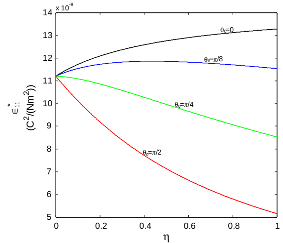
Fig. 7 The variations of \epsilon_{11}^* as a function of \eta at four different values of \theta_0 = 0, \pi/8, \pi/4, \pi/2 for a piezoelectric material BaTiO 3 containing two-dimensional insulating microcracks. The poling direction of the piezoelectric solid is along the x_2 -axis
