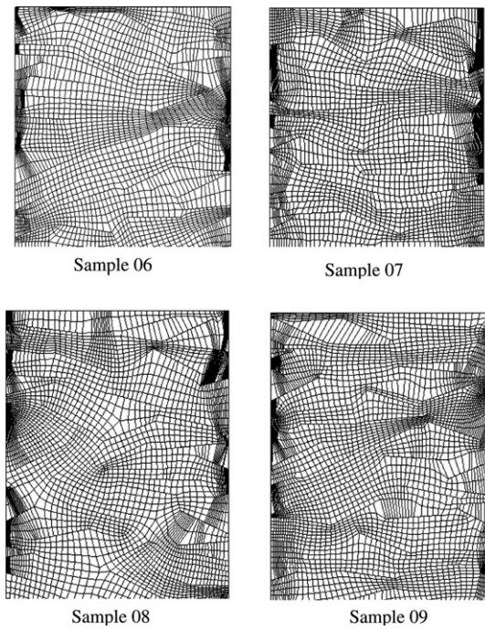
Fig. 5. The top part of finite element model of samples 06–09 ( \theta_0 = 30^\circ ).
