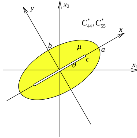
Fig. 1. The generalized self-consistent method.
