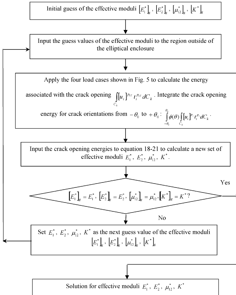
Fig. 9. Flow chart for calculating effective moduli of the medium in tension.
