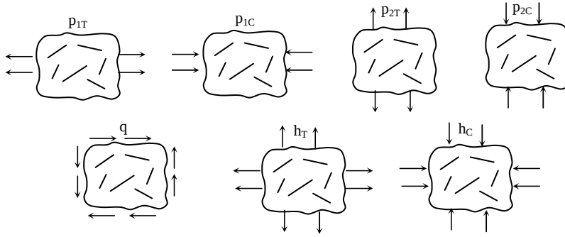
Fig. 7. Seven load cases for an initially stress-free medium.
