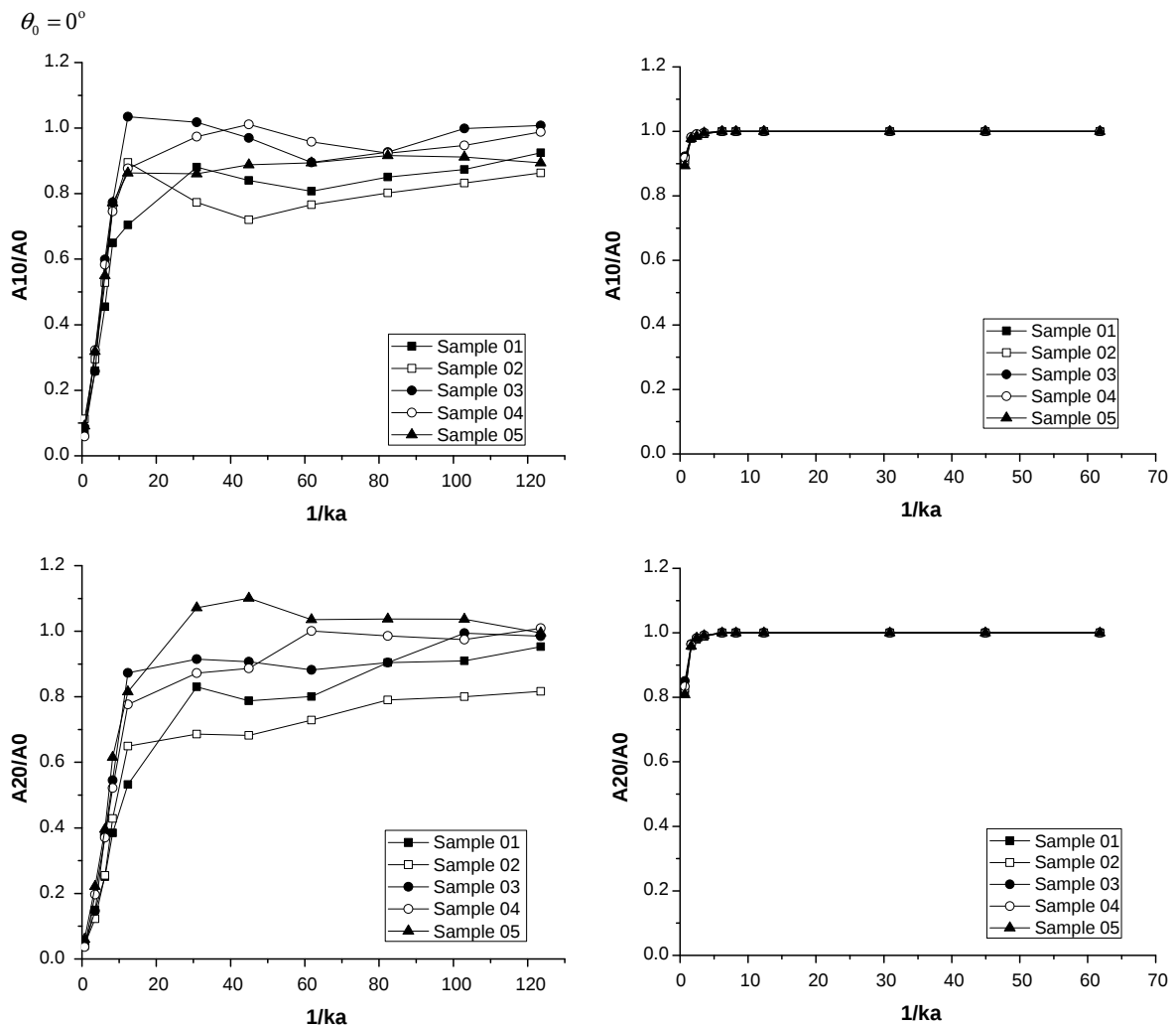
Fig. 13. Output signal strength vs. input effective wave number ( 1/ka ) for the models with \eta = 0.4 , \theta_0 = 0^\circ and 2a = 1 . Left column: Tensile waves output. Right column: Compressive waves output. First row: The normalized peak averaged stress measured at distance equal to 10. Second row: The normalized peak averaged stress measured at distance equal to 20.
