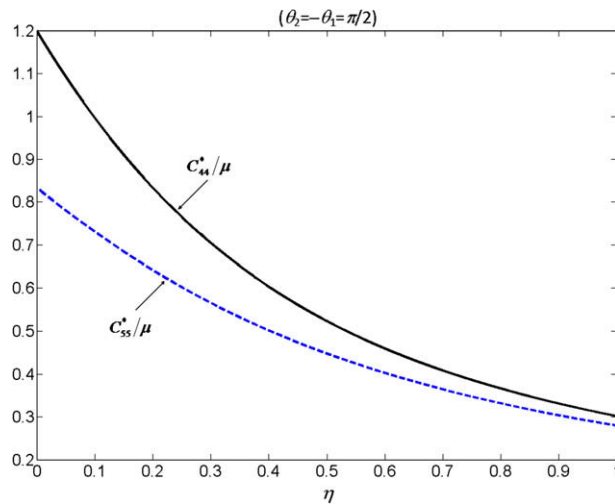
Fig. 10. The variations of C_{44}^* and C_{55}^* for an orthotropic solid C_{44} = 1.2\mu and C_{55} = 0.8333\mu containing randomly oriented cracks as functions of \eta .
