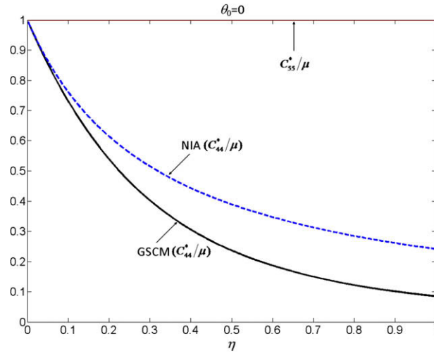
Fig. 2. The calculated C^*_{44} for an isotropic solid with perfectly aligned cracks.
