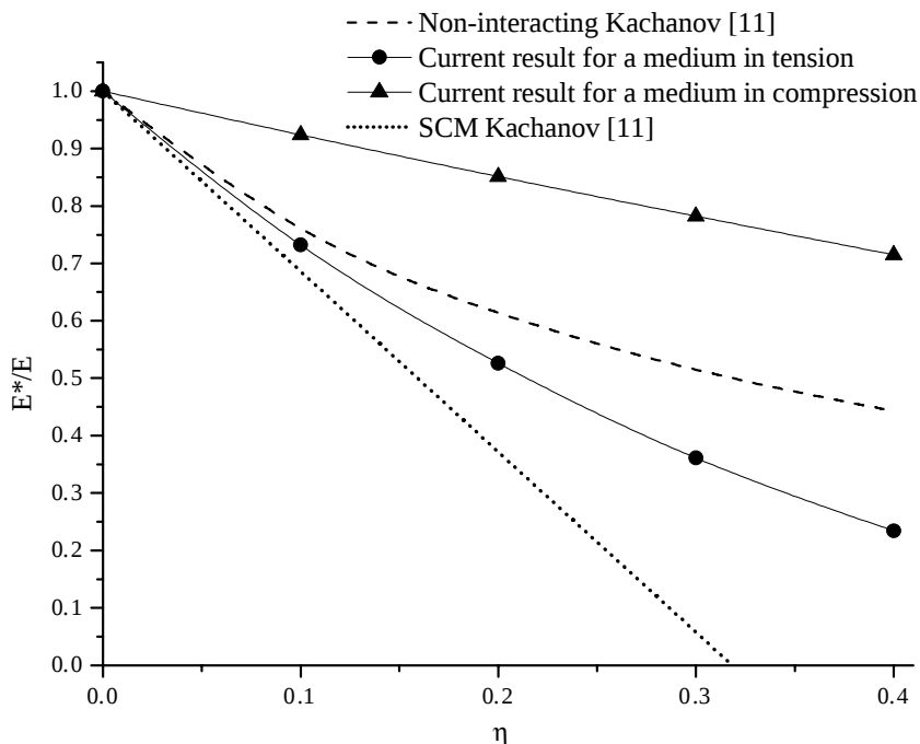
Fig. 11. Normalized effective Young's modulus for randomly distributed cracks vs. crack density.
