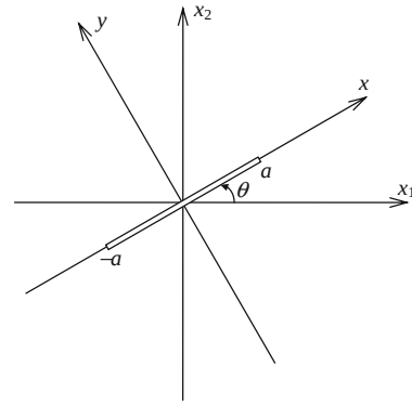
Fig. 1 A crack of half crack length a oriented at an angle \theta to the positive x_1 -axis
