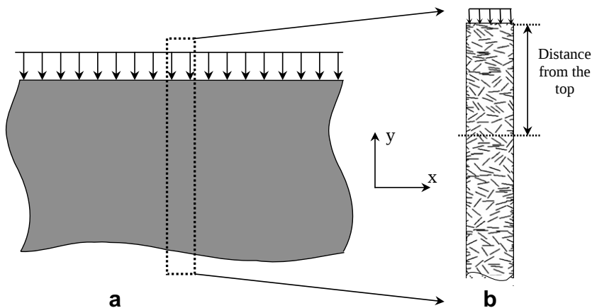
Fig. 2. Model schematics. (a) Time-dependent load is applied along the top boundary of the half plane. (b) A representative strip from the plane is used in the finite element simulation.
