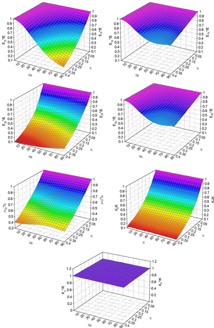
Fig. 15. Effective moduli of an initially stress-free medium.
