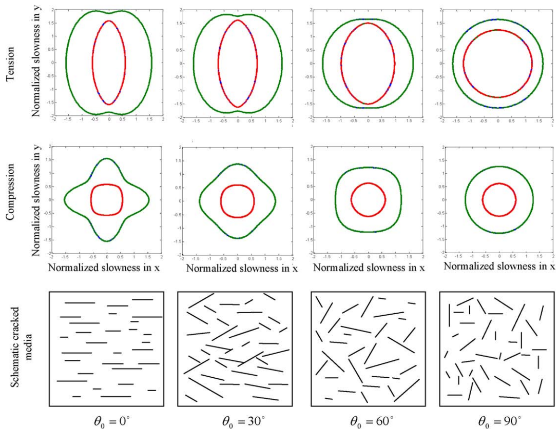
Fig. 17. Normalized slowness of cracked media under tension and compression. Crack density \eta = 0.4 . Outside lines: quasi-transverse wave; inside lines: quasi-longitudinal wave. All the lines are normalized by the slowness of transverse wave in virgin material.
