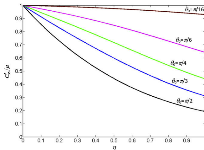
Fig. 5. The predicted values of C_{55}^* for a cracked isotropic solid as a function of \eta for five different values of \theta_0 .
