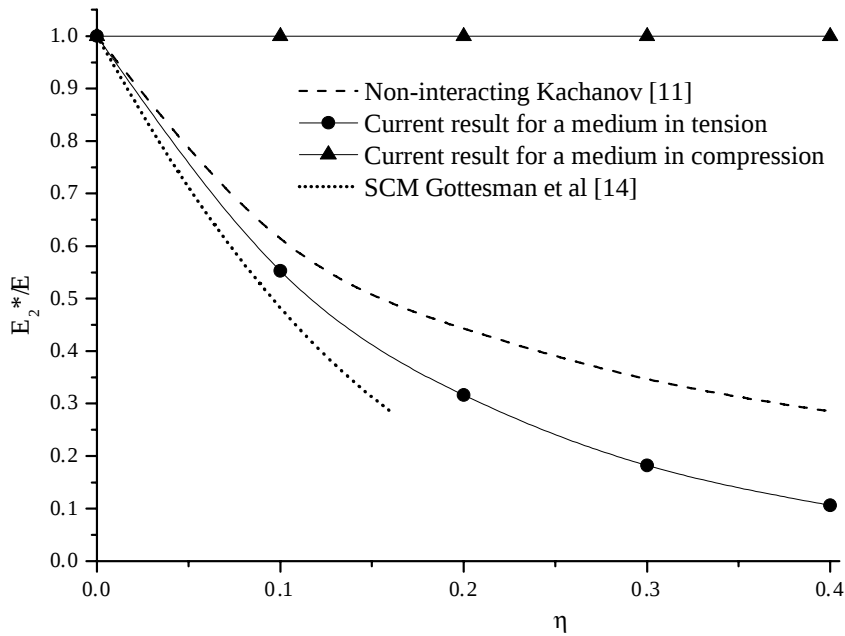
Fig. 12. Normalized effective Young's modulus, in the direction perpendicular to the cracks, for aligned cracks vs. crack density.
