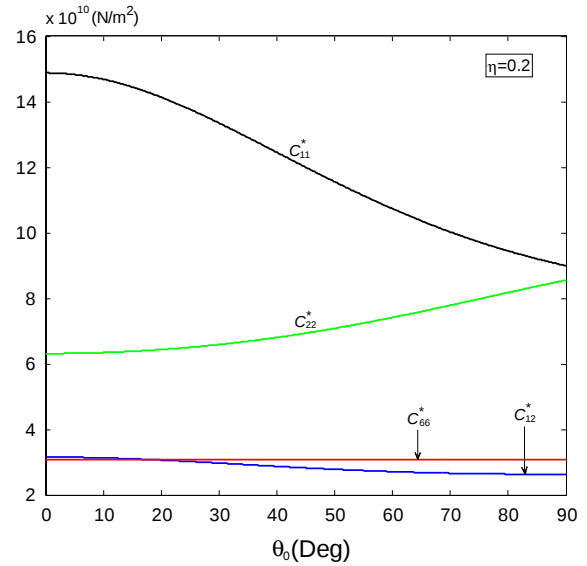
Fig. 3 The variations of the four effective elastic constants C_{11}^* , C_{22}^* , C_{12}^* and C_{66}^* as functions of \theta_0 with \eta = 0.2 for a piezoelectric material BaTiO 3 containing two-dimensional insulating microcracks. The poling direction of the piezoelectric solid is along the x_2 -axis
