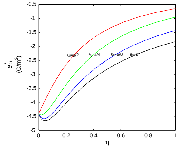
Fig. 6 The variations of e_{21}^* as a function of \eta at four different values of \theta_0 = 0, \pi/8, \pi/4, \pi/2 for a piezoelectric material BaTiO 3 containing two-dimensional insulating microcracks. The poling direction of the piezoelectric solid is along the x_2 -axis
