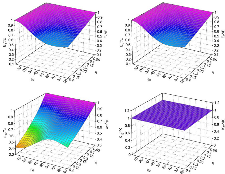
Fig. 14. Effective moduli of a medium in compression.
