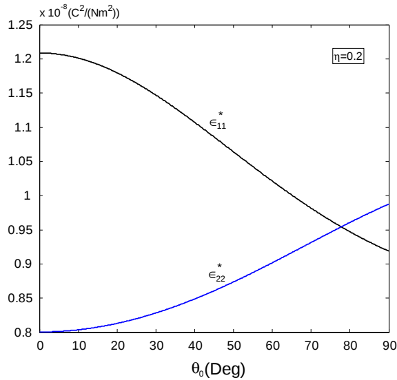
Fig. 5 The variations of the two effective dielectric constants \epsilon_{11}^* and \epsilon_{22}^* as functions of \theta_0 with \eta = 0.2 for a piezoelectric material BaTiO 3 containing two-dimensional insulating microcracks. The poling direction of the piezoelectric solid is along the x_2 -axis
