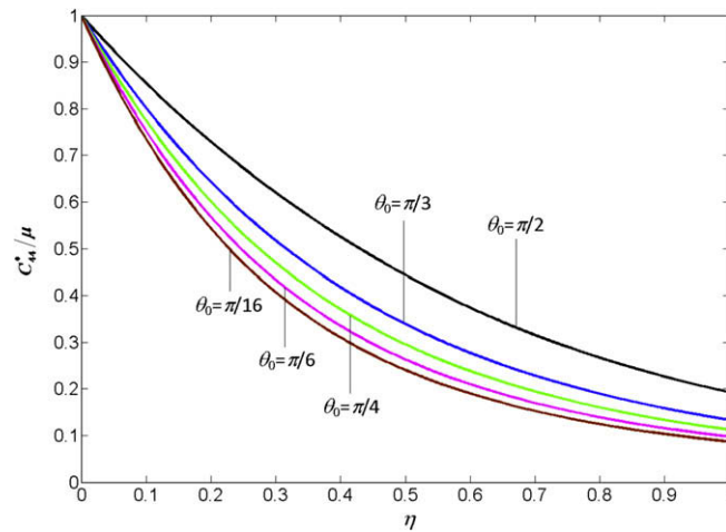
Fig. 4. The predicted values of C_{44}^* for a cracked isotropic solid as a function of \eta for five different values of \theta_0 .
