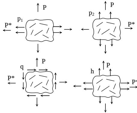
Fig. 5. Four load cases for medium in tension.
