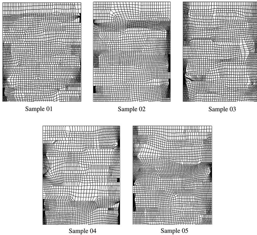
Fig. 4. The top part of finite element model of samples 01–05 ( \theta_0 = 0^\circ ).
