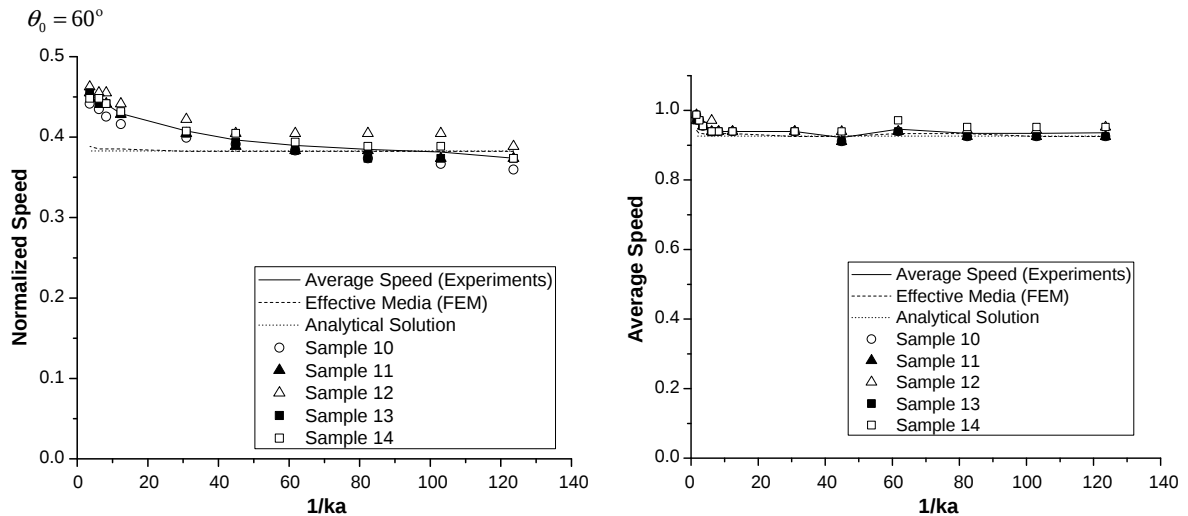
Fig. 10. Normalized wave speed vs. 1/ka for \theta_0 = 60^\circ . Left : speed of tensile waves. Right : speed of compressive wave.
