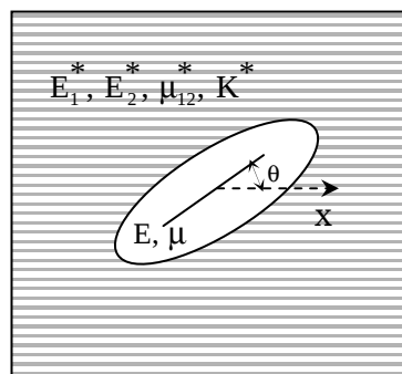
Fig. 2. Model of the crack problem from Santare et al. [19].
