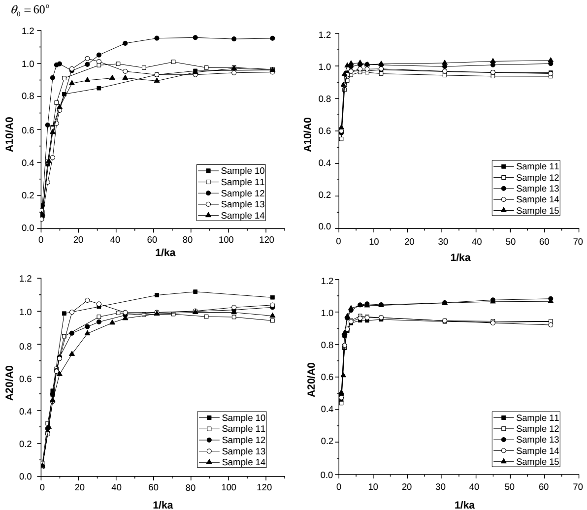
Fig. 15. Output signal strength vs. input wave length number ( 1/ka ) for the models with \eta = 0.4 , \theta_0 = 60^\circ and 2a = 1 . Left column: Tensile waves output. Right column: Compressive waves output. First row: The normalized peak averaged stress measured at distance equal to 10. Second row: The normalized peak averaged stress measured at distance equal to 20.
