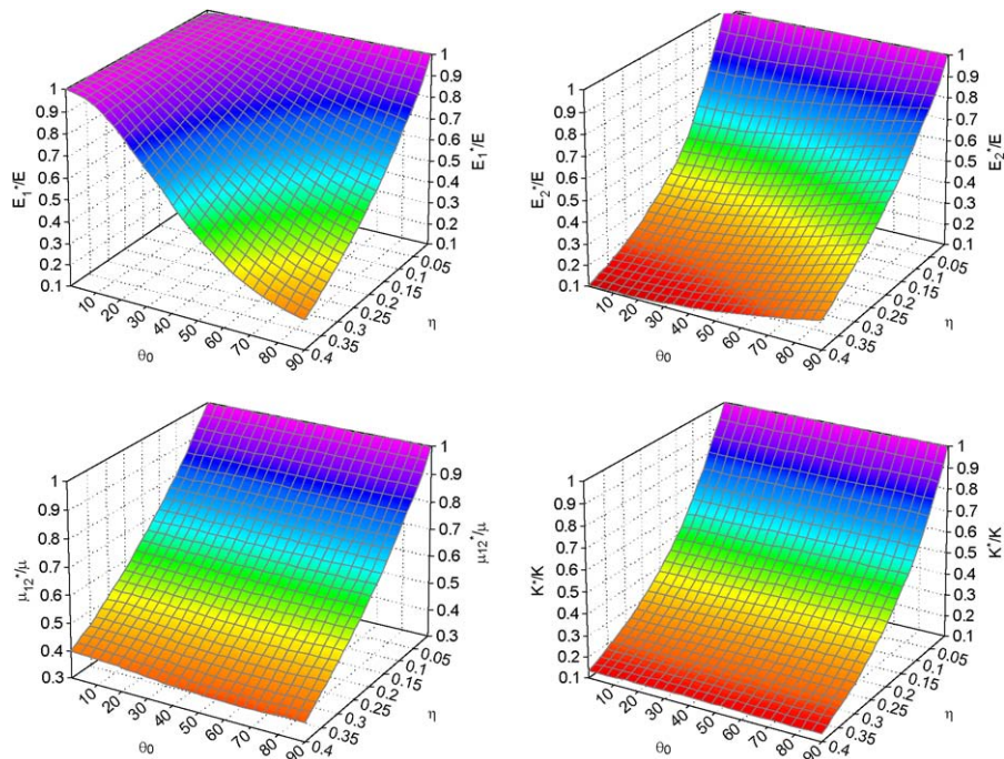
Fig. 13. Effective moduli of a medium in tension.
