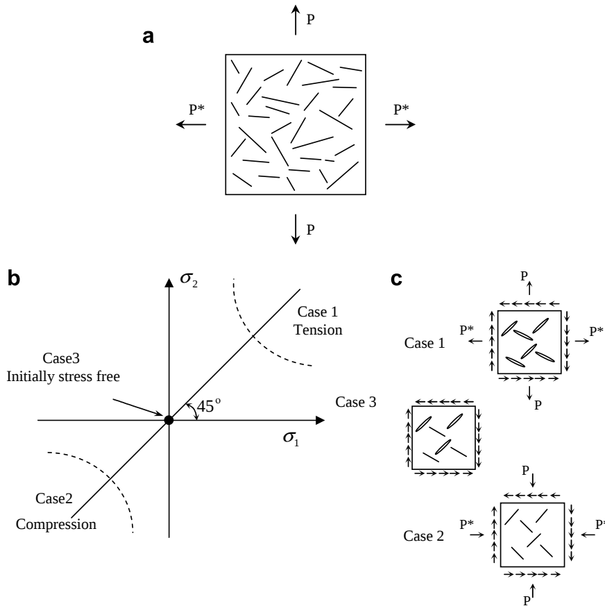
Fig. 4. (a) A cracked medium under bi-axial load. (b) Three different load cases. (c) Three cases with pure shear load increment.
