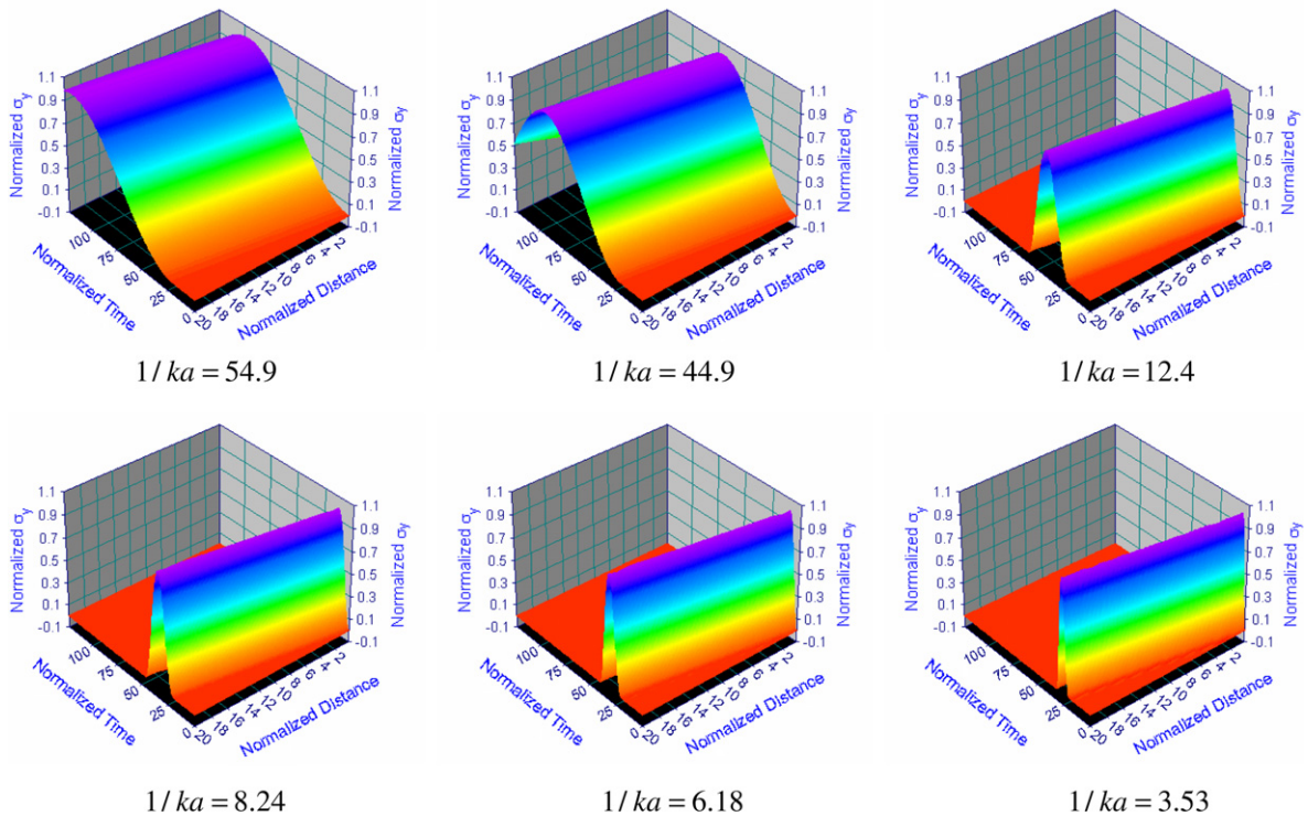
Fig. 12. Compressive waves with different effective wave number traveling in sample 05, \eta = 0.4 , \theta_0 = 0^\circ . Normalized \sigma_y is the average stress \sigma_y in the specific cross section normalized by the maximum average stress \sigma_y at distance equal to zero (the top boundary). The distance from the top is shown in Fig. 2b.
