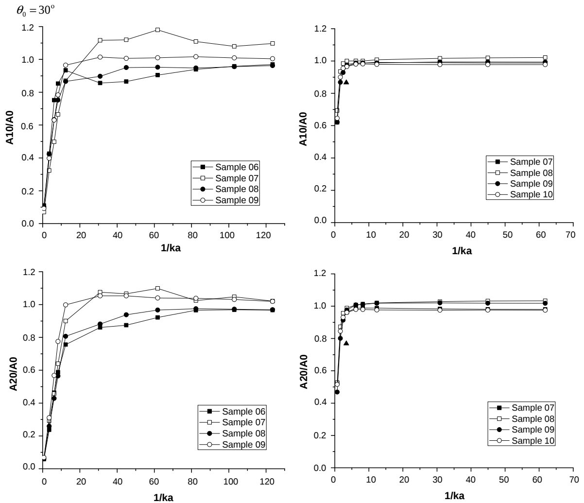
Fig. 14. Output signal strength vs. input wave length number ( 1/ka ) for the models with \eta = 0.4 , \theta_0 = 30^\circ and 2a = 1 . Left column: Tensile waves output. Right column: Compressive waves output. First row: The normalized peak averaged stress measured at distance equal to 10. Second row: The normalized peak averaged stress measured at distance equal to 20.
