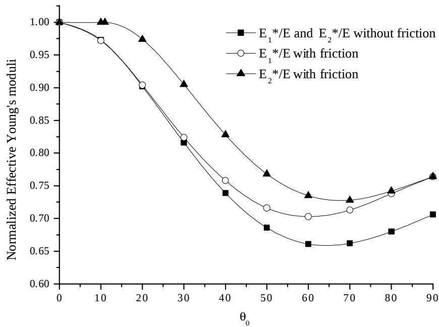
Fig. 16. Normalized E_{1C}^* , E_{2C}^* of initially stress-free media with and without friction. \eta = 0.4 and the friction coefficient equal to 0.2.
