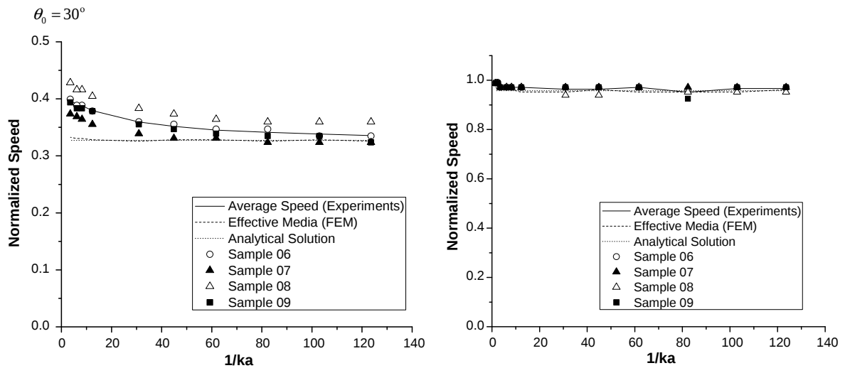
Fig. 9. Normalized wave speed vs. 1/ka for \theta_0 = 30^\circ . Left figure: speed of tensile waves. Right figure: speed of compressive wave.
