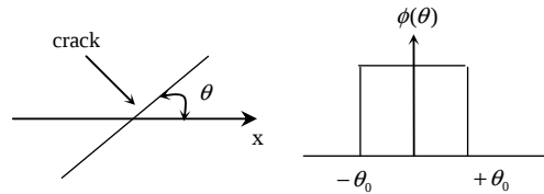
Fig. 1. Even distribution of crack orientation.
