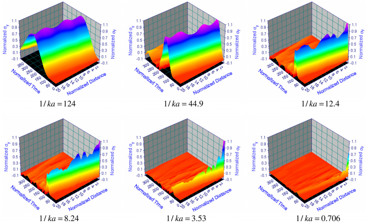
Fig. 11. Tensile waves with different effective wave number traveling in sample 05, \eta = 0.4 , \theta_0 = 0^\circ . Normalized \sigma_y is the average stress \sigma_y in the specific cross section normalized by the maximum average stress \sigma_y at distance equal to zero (the top boundary). The distance from the top is shown in Fig. 2b.
