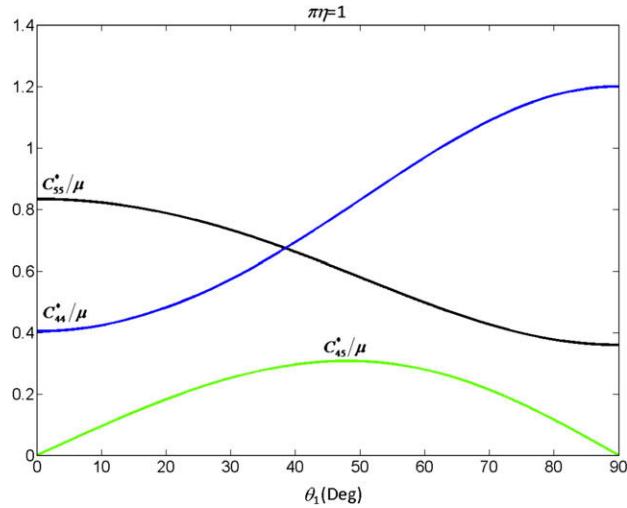
Fig. 9. The variations of C_{44}^* , C_{55}^* and C_{45}^* as functions of \theta_1 ( =\theta_2 ) for an orthotropic solid C_{44} = 1.2\mu and C_{55} = 0.8333\mu containing perfectly aligned cracks with \eta = 1/\pi .
