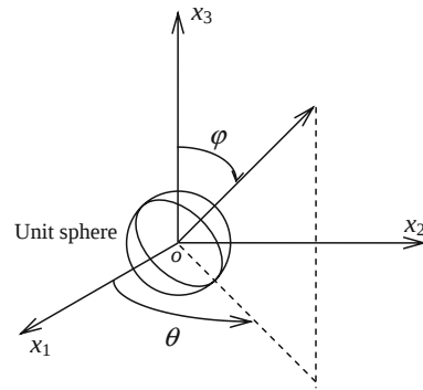
Fig. 8 Geometry of a penny-shaped crack
