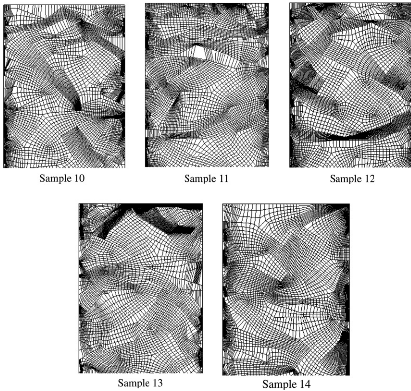
Fig. 6. The top part of finite element model of samples 10–14 ( \theta_0 = 60^\circ ).
