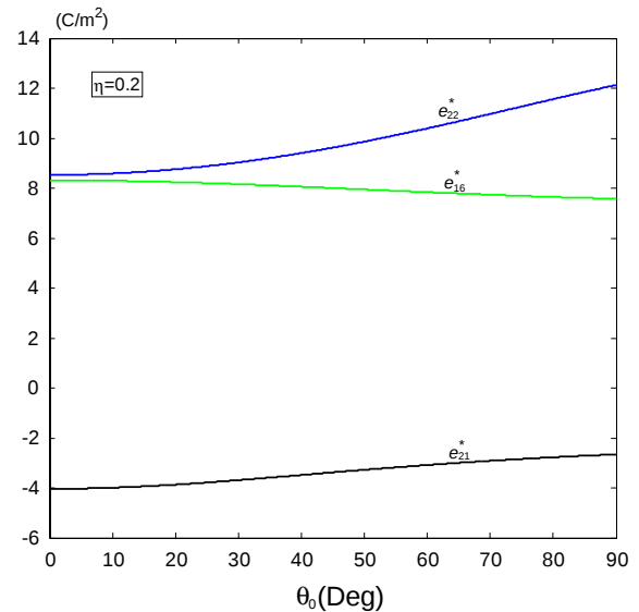
Fig. 4 The variations of the three effective piezoelectric constants e_{22}^* , e_{21}^* and e_{16}^* as functions of \theta_0 with \eta = 0.2 for a piezoelectric material BaTiO 3 containing two-dimensional insulating microcracks. The poling direction of the piezoelectric solid is along the x_2 -axis
