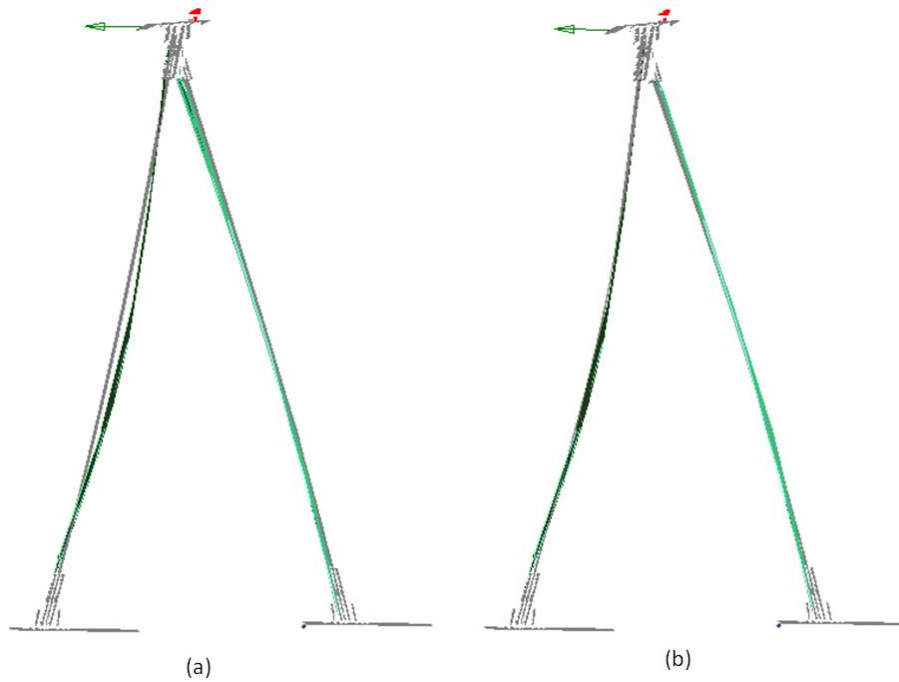
Figure 4.56: Solid Joined-wing - (a) Linear and (b) Non-linear FE Model under a 1,000 lb Load.
