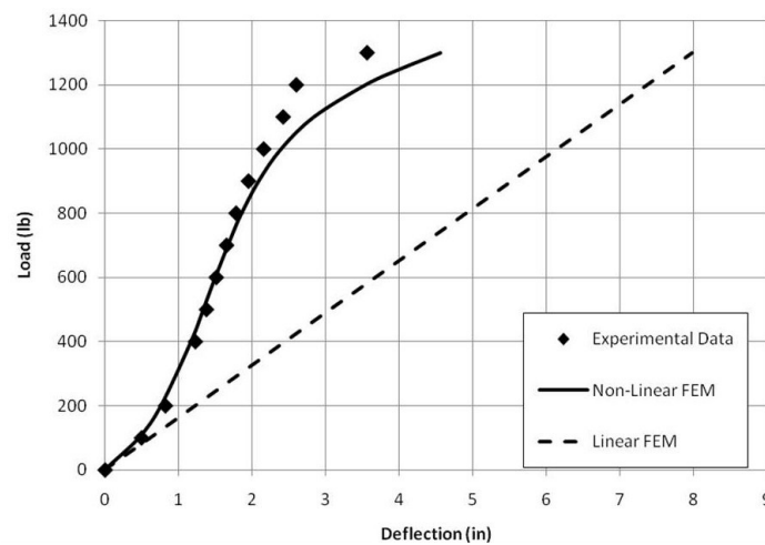
Figure 4.10: Solid Qualification - Transverse Bending - X Direction.
