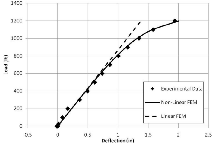
Figure 4.49: Solid Joined-wing - Point 4 - X-Direction.
