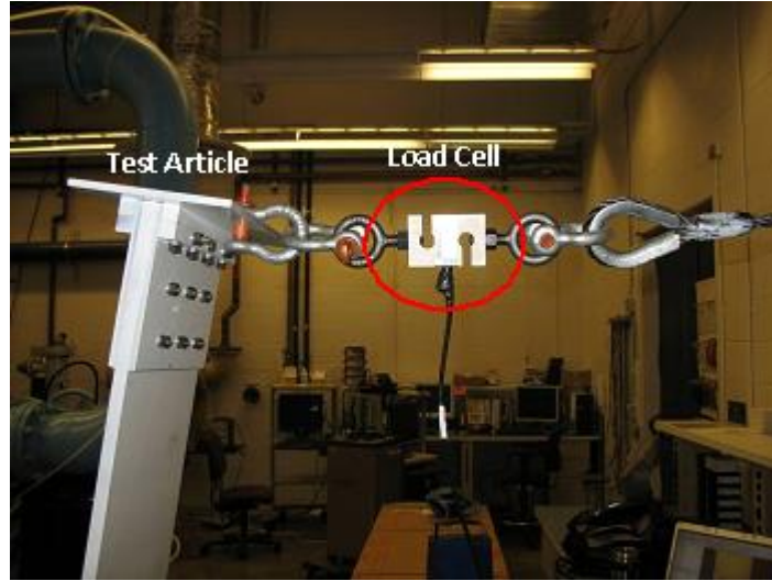
Figure 3.15: Load Cell.
