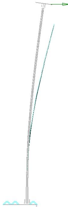
Figure C.3: Hollow Qualification - 20 lb Surface Matching - Linear.
