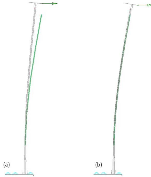
Figure 4.29: Hollow Qualification - 15 lb Surface Matching - (a) Linear and (b) Non-Linear.
