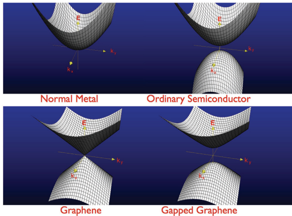
Fig. 4 Energy-momentum relations for different types of materials.
