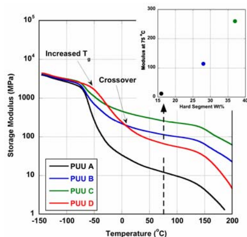
Figure 2. DMA storage moduli curves at 1 Hz for the various PUU materials. Inset shows the effect of HS content on the rubbery plateau modulus at 75 °C
