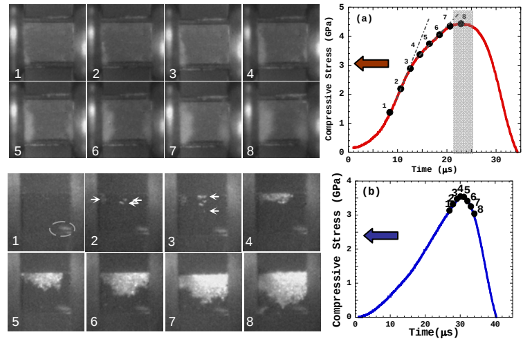
FIG. 3: Photographs from the high-speed camera of the dynamic failure process in (a) confined and (b) unconfined AlON along with the respective stress evolution curves on the right. The interframe and the exposure time for the confined case are 2\ \mu\text{s} and 200\ \text{ns} , respectively and for unconfined case are 1\ \mu\text{s} and 100\ \text{ns} , respectively (circled region in Frame-1 (and similar for other frames) in 3 (b) shows the flow of the lubricant). Note the damage evolution for the confined case is slower and the region exhibits lower contrast in the photos compared with that of unconfined case; stress evolution curve also suggest a non-linear material response (accompanied by a higher peak stress) which is not evident for the unconfined case.
