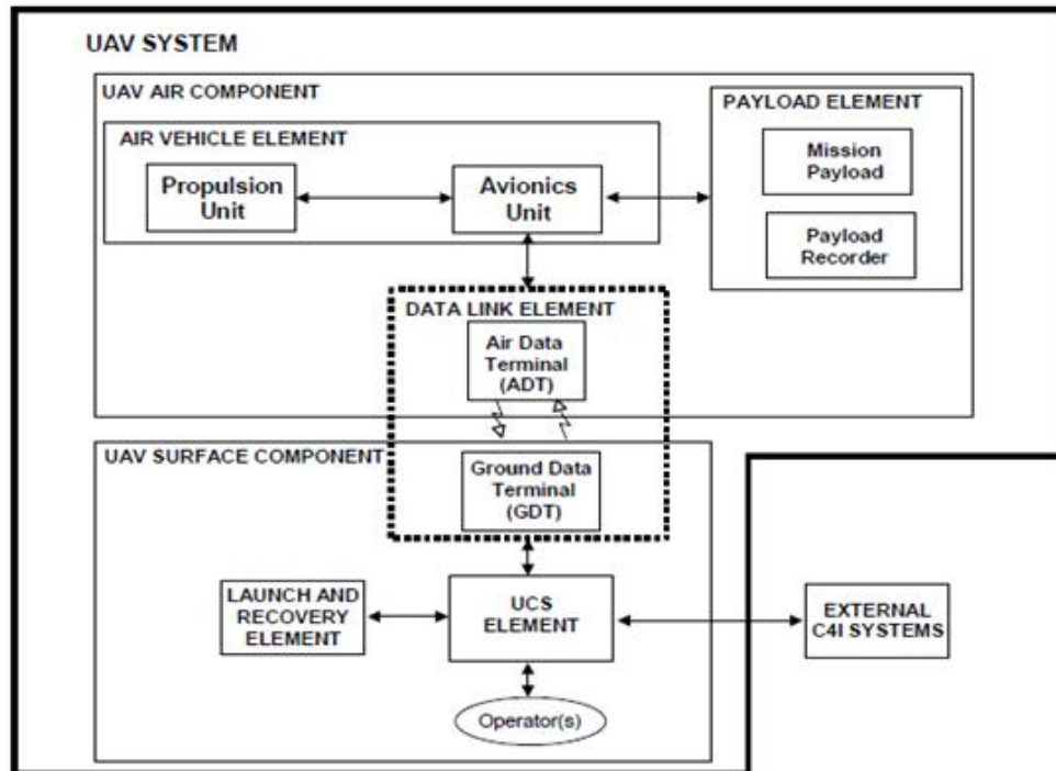
Figure 5. Top-Level UAS Architecture as Defined by STANAG 4586
