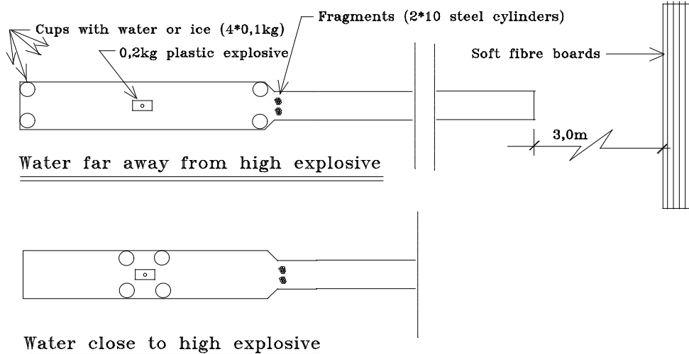
Figure 3. Set up in experiments with fragments.
