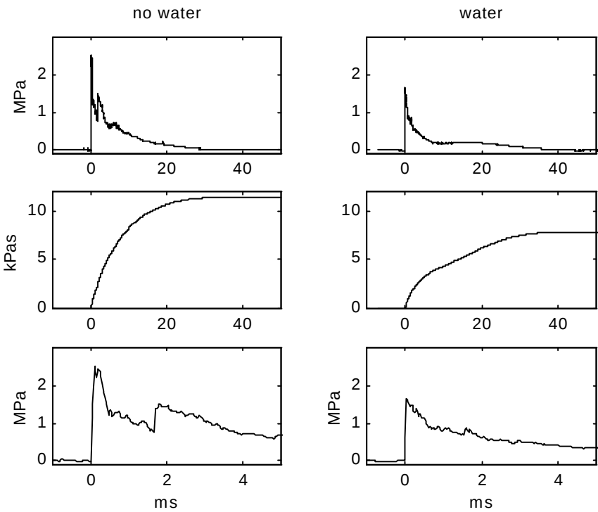
Figure 8. Registrations from Mp2 , Q = 200\text{ g} , W = 0 and 400\text{ g} (alternative 3).
