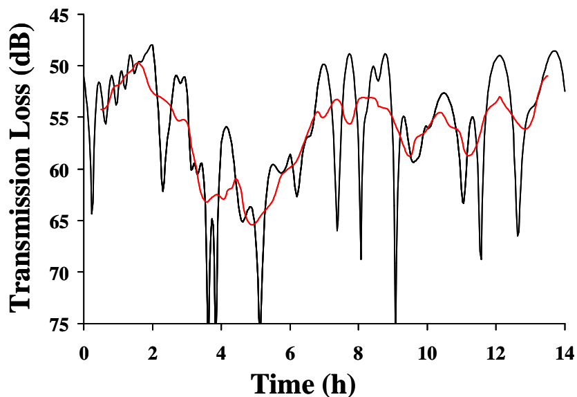
Fig. 9. Transmission loss as a function of time at 10kHz. depth=53m, range=2km.
