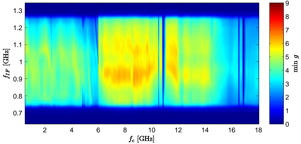
Figure 4.75 Minimum gain of the sixteen downconverter channels, at each point in the frequency spectrum.
