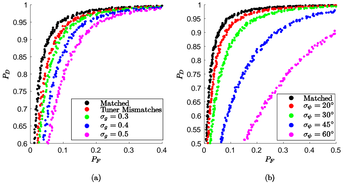
Figure 6.1 Simulated ROC curves for a 16-channel receiver, with A_s = 3 \mu\text{V} , f_{in} = 4.5 \text{ GHz} , \sigma_w = 10 \mu\text{V} , T_2 - T_1 = 2.2 \text{ ns} , \text{SNR}=0.09 ( -10.5 \text{ dB} ), and noise bandwidth from 1-8 GHz. (a) Results of Simulations 1-5 (gain mismatches). (b) Results of Simulations 1 and 6-9 (phase mismatches). The simulation parameters are given in Table 6.1. Combined effects of gain and phase mismatches are not shown.
