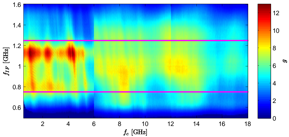
Figure 4.8 Tuner 4 gain at -3°C (linear scale).
