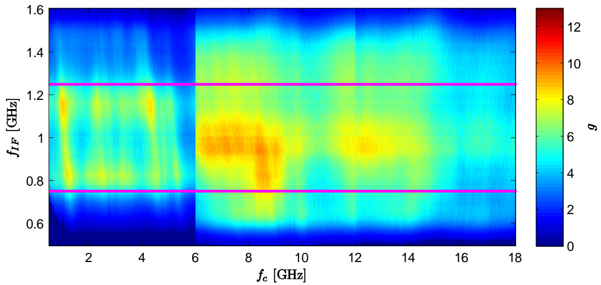
Figure 4.14 Tuner 6 gain at 50°C (linear scale).
