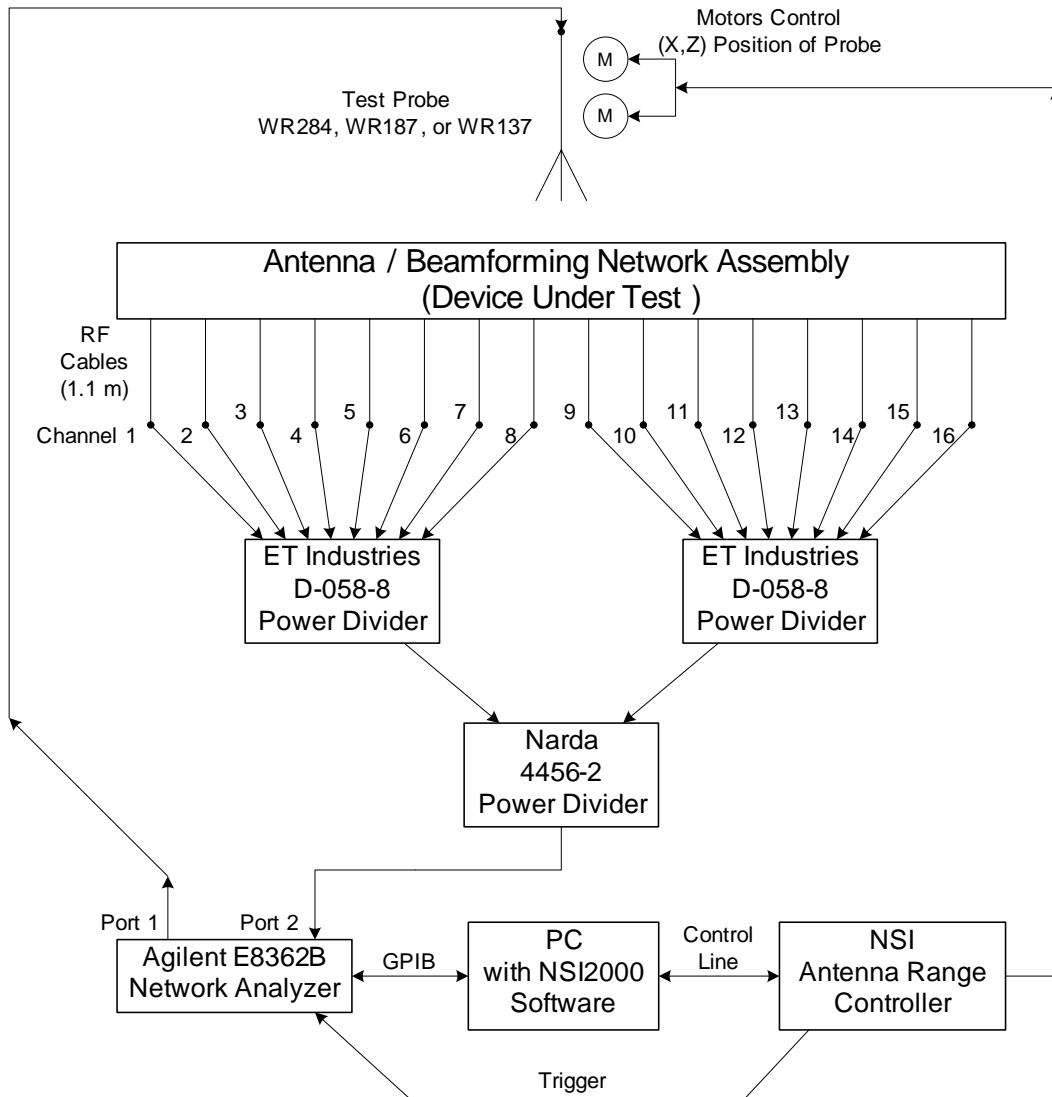
Figure 3.9 Test setup for measuring the antenna pattern of the entire MCWESS antenna. The CSA/BN assembly and test probe were inside a near-field anechoic chamber. The power "dividers" are reversed, and used as summing devices.
