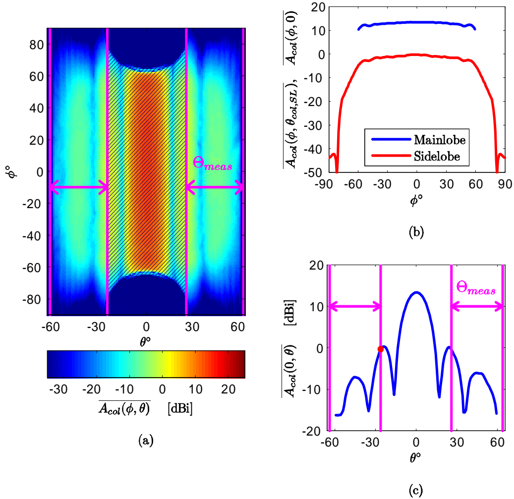
Figure 5.26 Illustration of how \Theta_{meas} is used to find FNBW_\phi by looking at a sidelobe. (a) Plot of \overline{A_{col}(\phi, \theta)} . We can not determine FNBW_\phi from the main lobe, because no data are available at those angles. (b) Azimuth cut, showing the main lobe \overline{A_{col}(\phi, 0)} and the sidelobe \overline{A_{col}(\phi, \theta_{col, SL})} . The first nulls of the sidelobe are sometimes well-shaped, as in this figure. In all such cases, FNBW_\phi \approx 162^\circ , regardless of frequency. (c) Elevation cut. The angle \theta_{col, SL} is highlighted with the red dot. Remember that none of these plots are of a single antenna pattern, but rather are the average of all sixteen superelement patterns.
