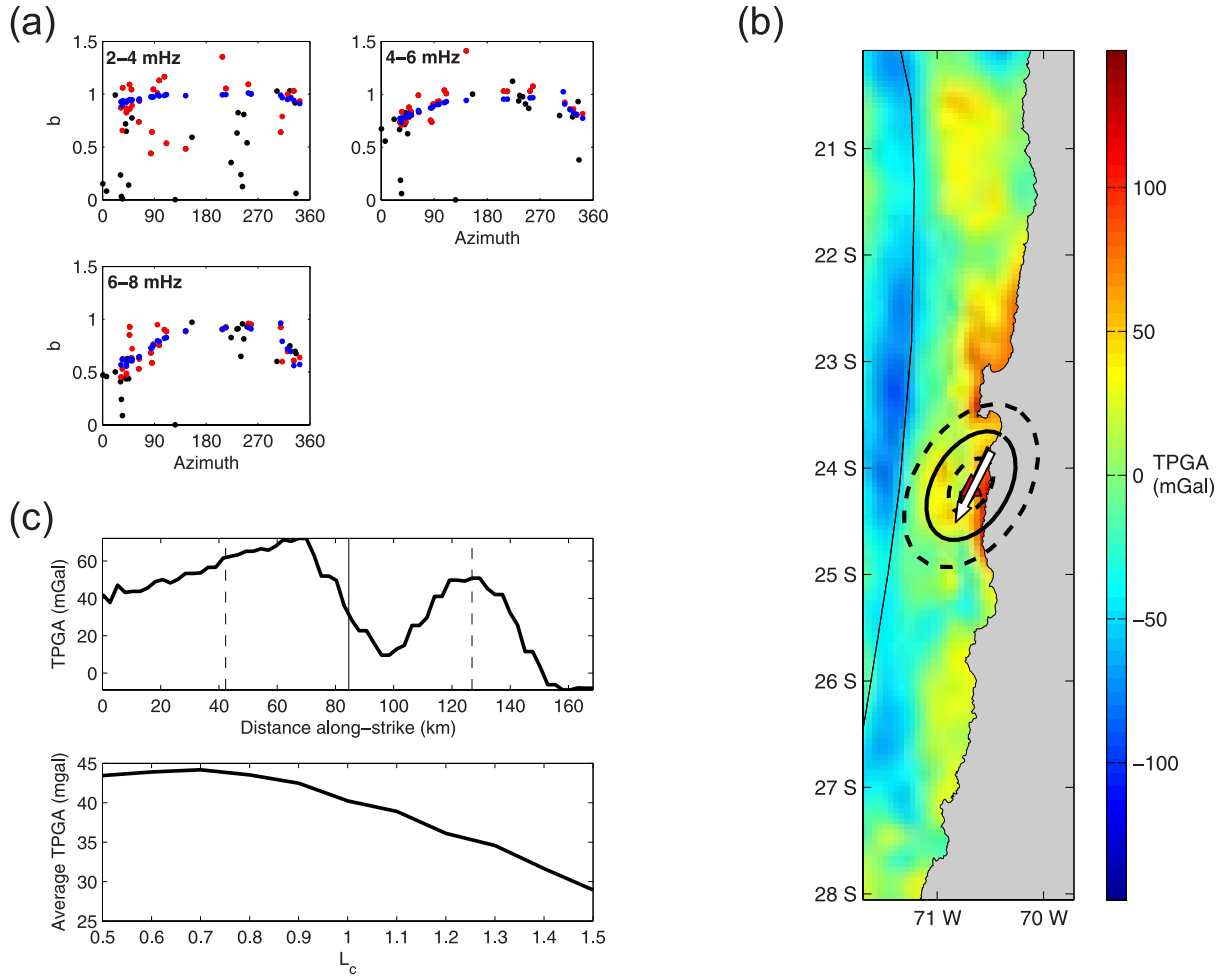
Figure B5. Measurements and results for event 19950730 in Chile using a M_w 5.9 aftershock that occurred on 3 August 1995 as an EGF. (a) See Figure B4 for symbol explanation. Note the large amount of scatter in the 2–4 mHz band. (b) See Figure 4 for symbol explanation. Compared to the TGF results, the ellipse has rotated by \sim 14^\circ but remains oblique to the strike of the trench. (c) See Figure 4 for symbol explanation. Although these plots have changed slightly from the original results, the overall conclusion remains the same qualitatively.
