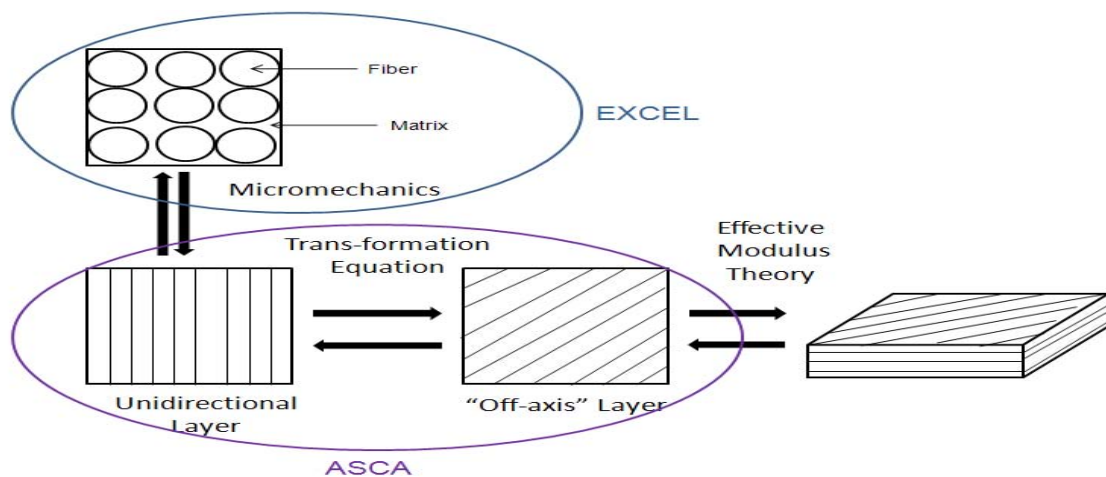
Figure 4-7 Analyzing composites
