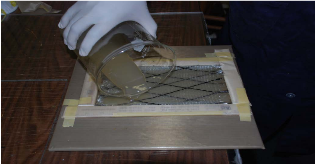
Figure 3-8 Pouring resin
