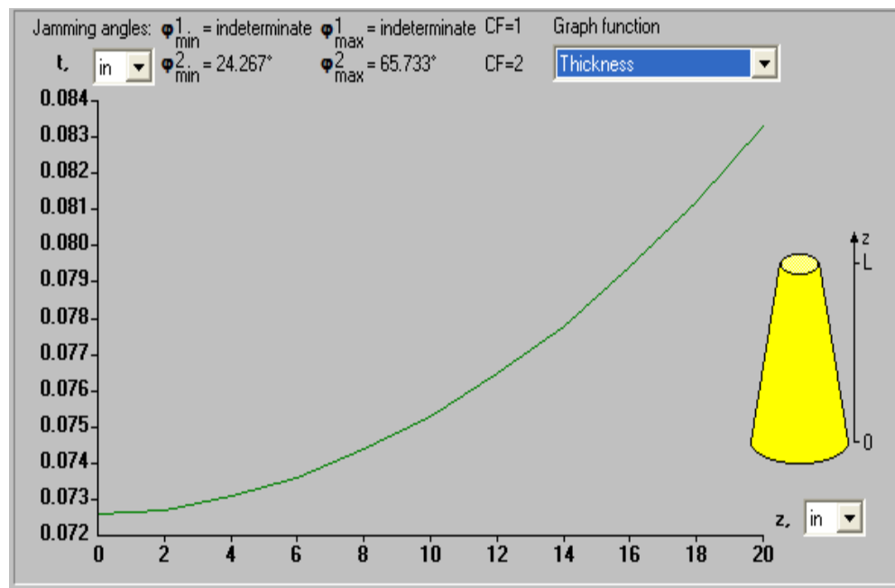
Figure C-2 Braids analysis of thickness
