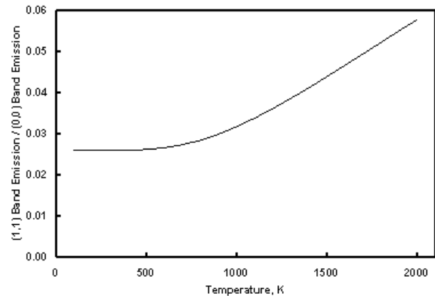
Figure 21. Ratio of (1,1) to (0,0) N_2^+ B-X Emission vs. Vibrational Temperature.
