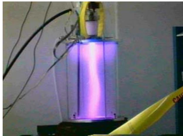
Figure 8. Photograph of 27-kV Pulsed E-Beam Gun in Operation Using N_2 at 70 mtorr.
