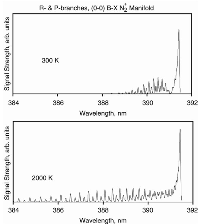
Figure 18. Calculated N_2^+ (0-0) Emission Spectra at 300 and 2,000 K (Instrumental Width: 0.05 nm).
