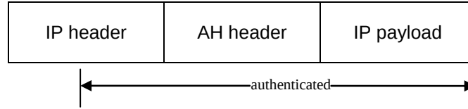
Figure 18: AH Transport Mode encapsulation [26]
