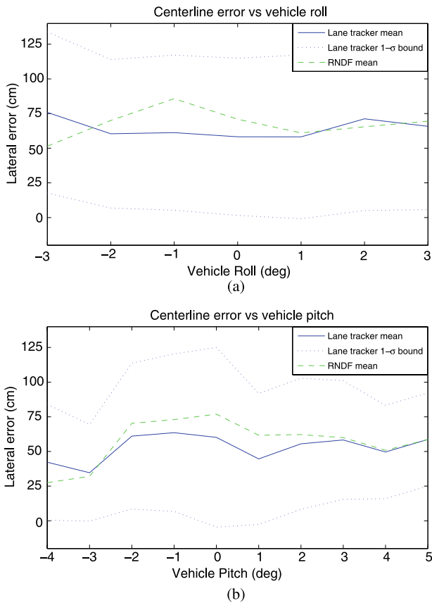
Fig. 17 Centerline error of our system and the RNDF prior as a function of vehicle roll and pitch, with 1- \sigma bounds
