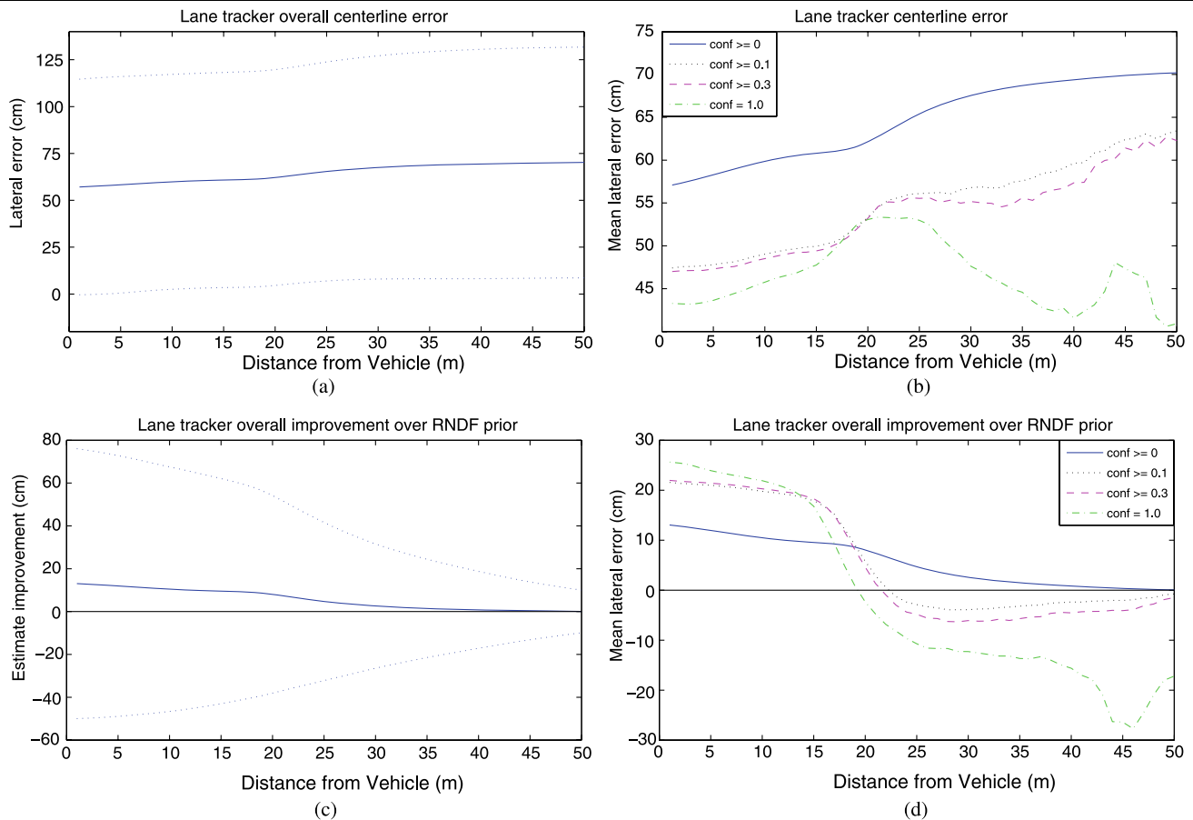
Fig. 14 Centerline error as a function of distance along lane. (a) Mean error with 1-\sigma bounds. (b) As system confidence increases, its accuracy improves. (c) Mean improvement over the RNDF with 1-\sigma
