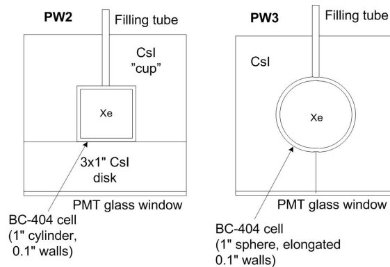
Figure 1. Geometries of phoswich well detectors studied. Left: 1st well prototype (PW2). Right: 2nd well prototype and production detectors (PW3-PW7).
