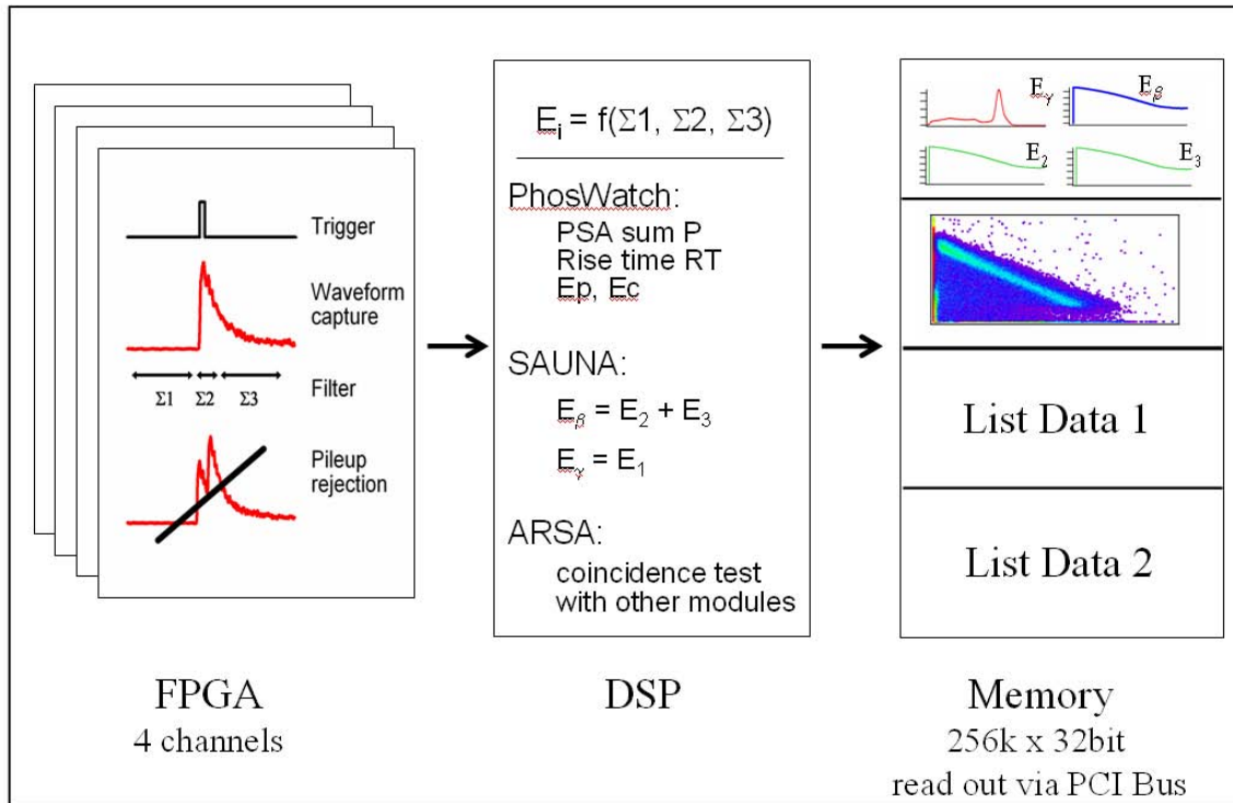
Figure 4. Block diagram of processes in the Pixie-4. After digitization, pulses are detected in an FPGA that also computes energy filter sums. A DSP computes the energy E , analyzes the captured waveforms to compute PSA parameters, and computes E_c and E_p . Energy histograms and list mode data are stored in on-board memory and can be read out to the host PC in fast block transfers.
