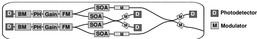
Fig.1. Functional schematic of chip.
