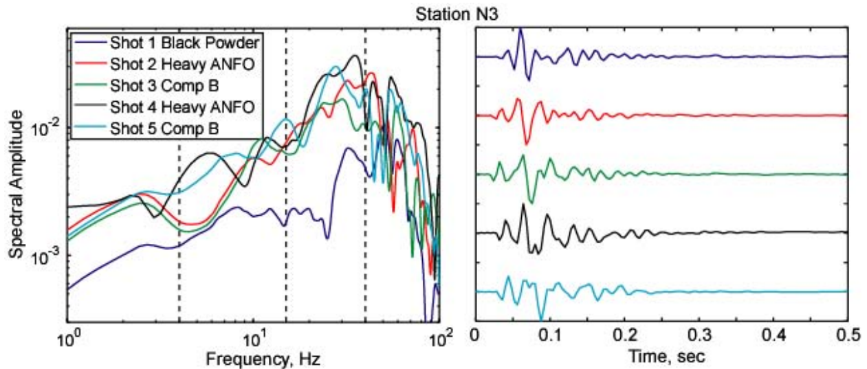
Figure 94. Spectral amplitudes of the five explosions (left) recorded on the vertical component of station N3 (shots 1-3 \text{SD} \approx 15 \text{ m/kg}^{0.5} , shots 4-5 \text{SD} \approx 11 \text{ m/kg}^{0.5} ). The vertical dashed lines delineate the different USBM vibration limit frequency ranges. On the right are the seismic waveforms recorded for each shot at station N3.
