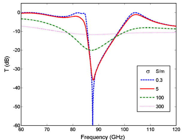
Fig. 4. Calculated transmission spectra for simulation model 2 as a function of the conductivity of the thin photoconducting film.
