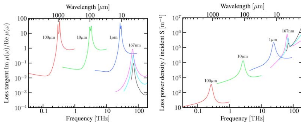
Fig. 3 (online colour at: www.pss-b.com ) Magnetic loss tangent \text{Im } \mu(\omega)/\text{Re } \mu(\omega) is shown for a single-gap SRR as a function of frequency for different sizes L of the SRR unit cell: L = 100 \mu\text{m} (red), 10 \mu\text{m} (green), 1 \mu\text{m} (blue), 167 \text{ nm} (pink), 100 \text{ nm} (turquoise) and 50 \text{ nm} (black).
