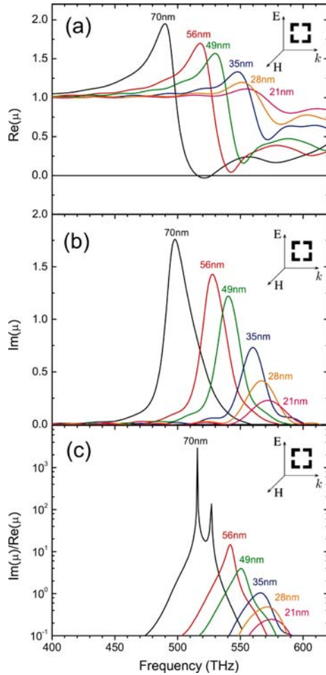
Fig. 9 (online colour at: www.pss-b.com ) Real part (a) and imaginary part (b) of the resonant effective permeability \mu(\omega) and loss tangent (c) \text{Im}(\mu(\omega))/\text{Re}(\mu(\omega)) are shown for a four-gap SRR as function of frequency for different sizes L of the SRR unit cell: L = 70 nm (black), 56 nm (red), 49 nm (green), 35 nm (blue), 28 nm (orange) and 21 nm (magenta). In part (a), the magnitude of magnetic resonance reduces as L scales down, and only L = 70 nm (black curve) shows a negative \mu at around 520 THz. All the frequencies below 520 THz show negative \mu .
