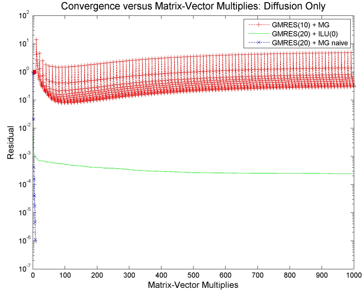
Figure C-5: Convergence history of \text{GMRES}(m) solver using different preconditioners. Here no preconditioner is used to precondition the \text{GMRES}(m) smoother for a pure diffusion case with a proper p -MG implementation. Fourth order basis functions are used on the fine grid.
