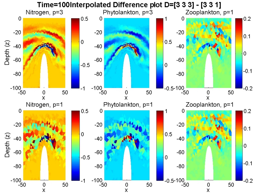
Figure 4-15: Difference between fields calculated using a third order basis for Zooplankton minus using a first order basis for Zooplankton. Nitrogen and Phytolankton both use third order bases and the difference in [\mu\text{mol}] projected onto first order bases is plotted on the bottom row. Color bars shown are in [\mu\text{mol}] .
