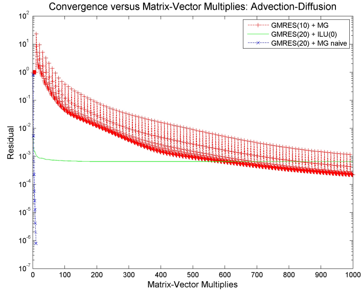
Figure C-6: Convergence history of \text{GMRES}(m) solver using different preconditioners. Here no preconditioner is used to precondition the \text{GMRES}(m) smoother for advection-diffusion case with a proper p -MG implementation. Fourth order basis functions are used on the fine grid.
