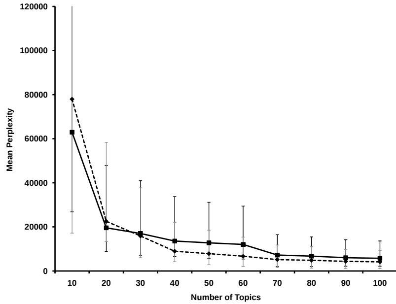
Figure 4.10: Mean Perplexity results for the IED collection.
