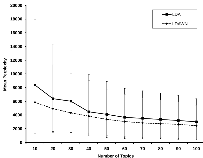
Figure 4.8: Mean Perplexity results for the NIPS collection.
