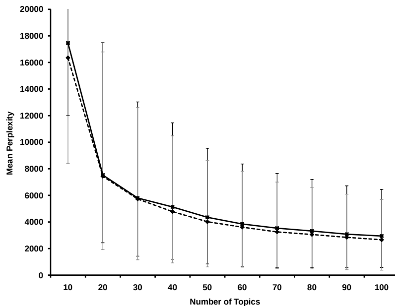
Figure 4.7: Mean Perplexity results for the 20 Newsgroups collection.
