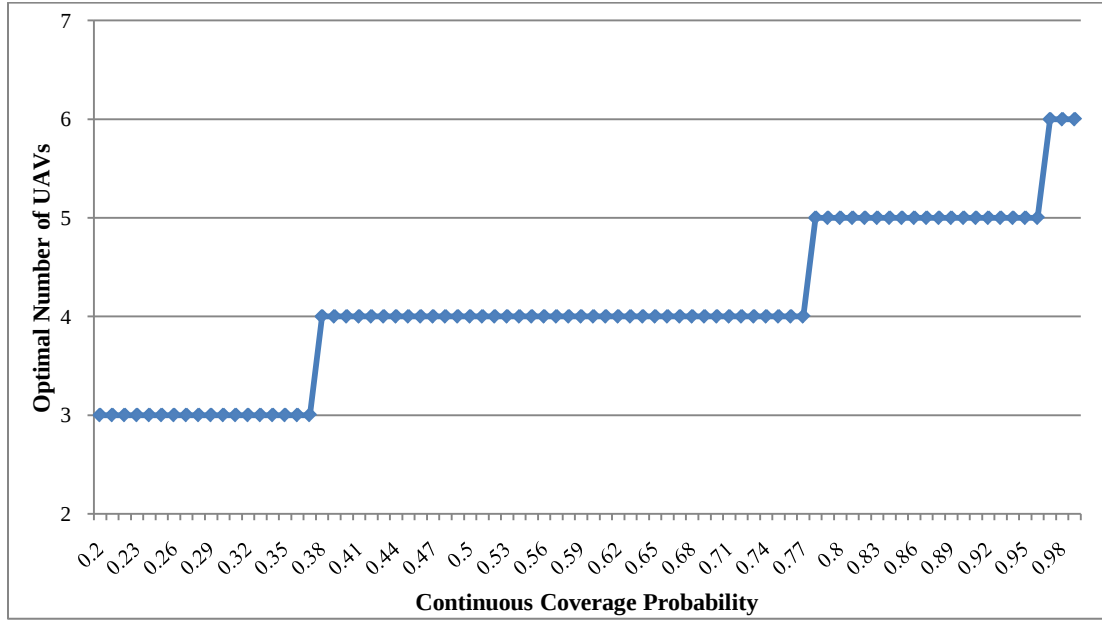
Figure 25. Optimal Number of UAVs vs. Threshold Coverage Probability
