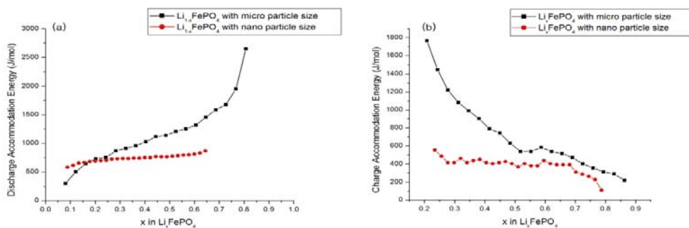
Figure 6. Accommodation energy of \text{LiFePO}_4 with different particle size during (a) discharge and (b) charge
