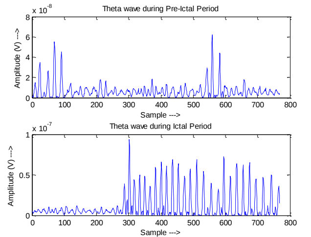
Figure 3: Theta wave during Pre-Ictal and Ictal Periods
