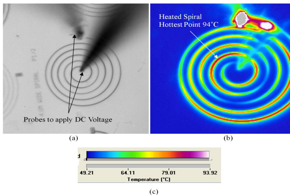
Figure 43 6 \mu m Spiral, Poly1-Poly2 stack, 10V DC, temperature range 49 to 93.9°C
