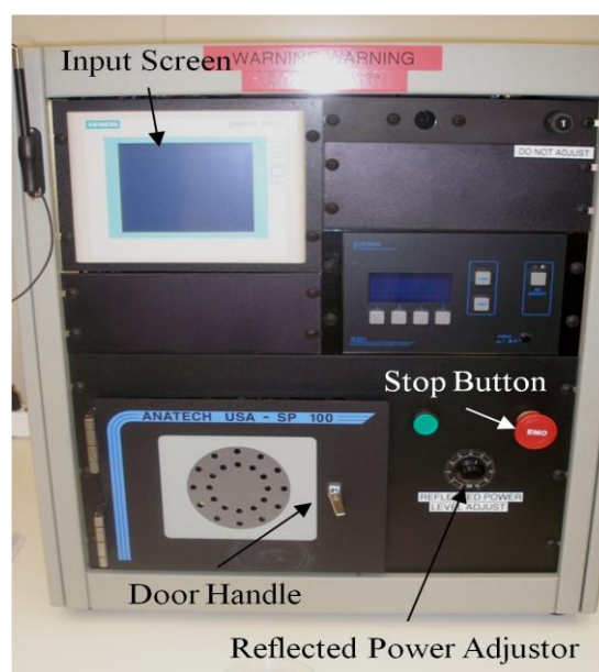
Figure 21 Plasma Asher
