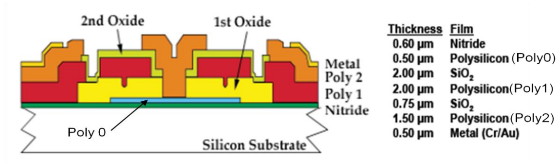
Figure 9 PolyMUMPs™ fabrication process, film layers listed in order of deposition and growth and labels correspond to layers [7]
