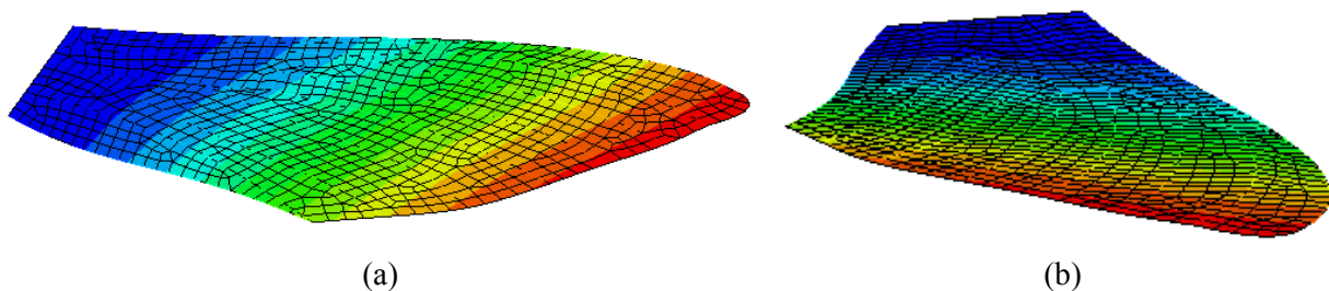
Figure 57: First modeshape (41 Hz) of a flat, FE wing with added veins, shown from an isometric view (a) and a tip view (b). Color bands denote displacement.
