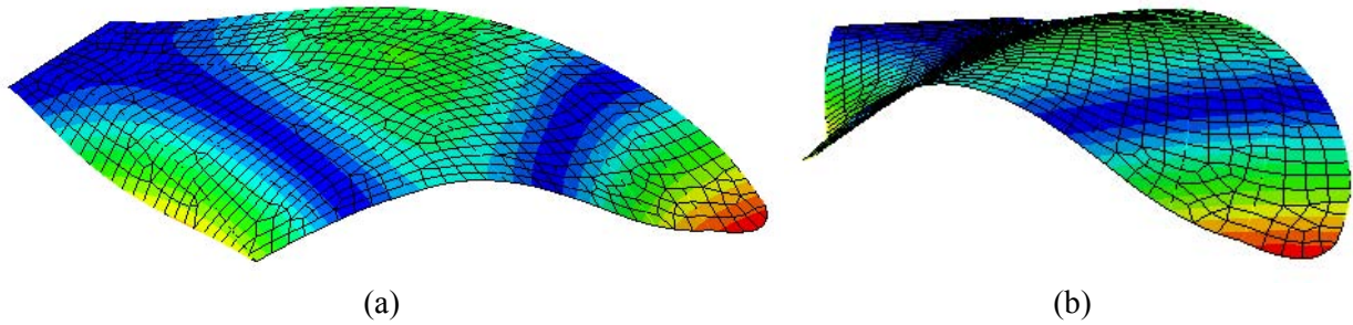
Figure 60: Fourth modeshape (308 Hz) of a flat, FE wing with added veins, shown from an isometric view (a) and a tip view (b).
