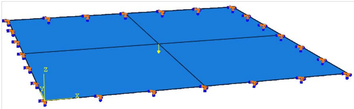
Figure 40: Rectangular structure comprised of membrane elements, with a central load.
