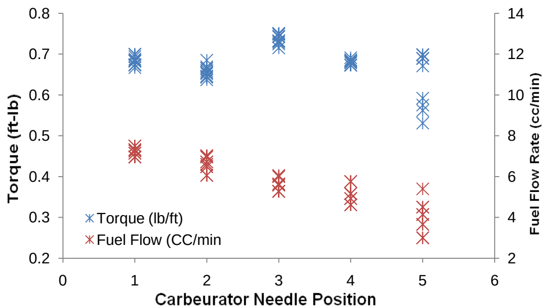
Figure 84. Raw data for varied carburetor needle position n-Heptane at 300K, 4000 RPM, 100% throttle and stock timing
