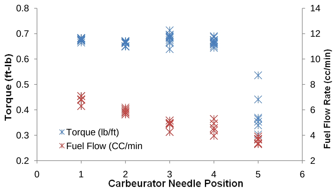
Figure 87. Raw data for varied carburetor needle position n-Heptane at 333K, 4000 RPM, 100% throttle and stock timing
