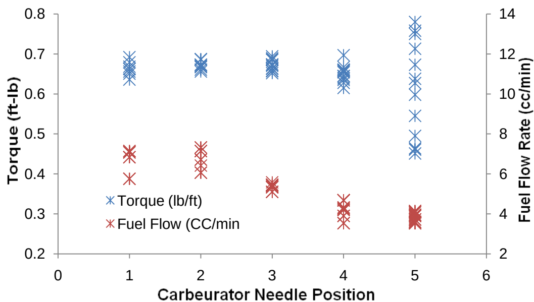
Figure 85. Raw data for varied carburetor needle position n-Heptane at 311K, 4000 RPM, 100% throttle and stock timing
