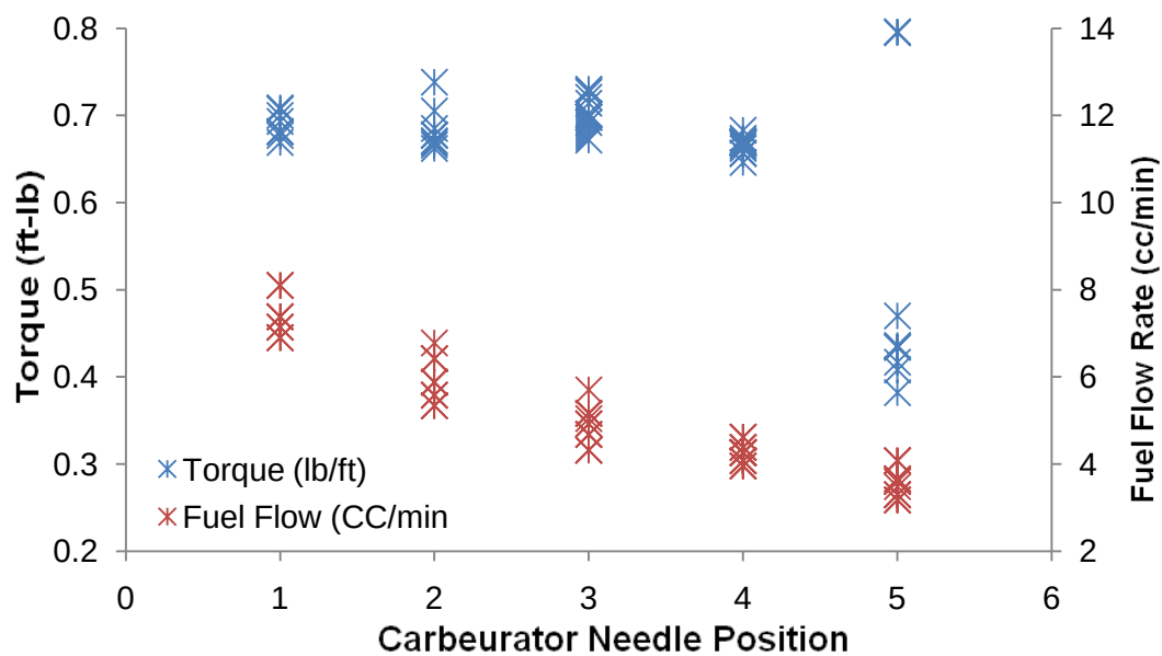
Figure 86. Raw data for varied carburetor needle position n-Heptane at 322K, 4000 RPM, 100% throttle and stock timing
