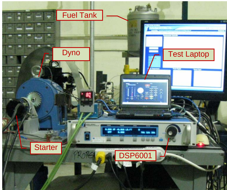
Figure 6. Dynamometer setup
