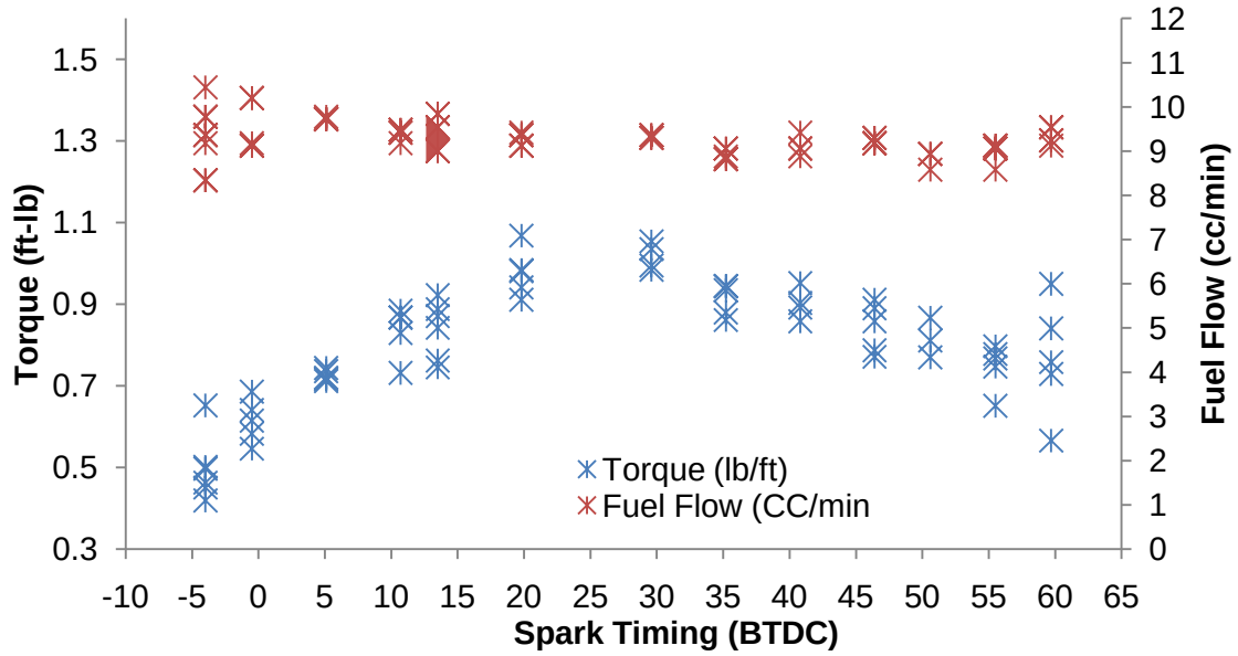
Figure 60. Raw torque and fuel flow for varied spark timing for n-Heptane at 5700 RPM
