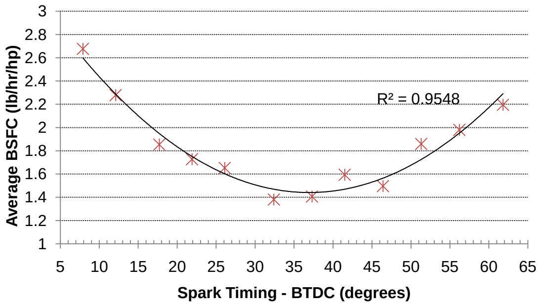
Figure 73. Average BSFC vs. spark timing for n-Heptane at 5000 RPM
