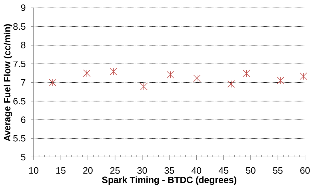
Figure 69. Average volumetric fuel flow rate vs. spark timing for n-Heptane at 3500 RPM
