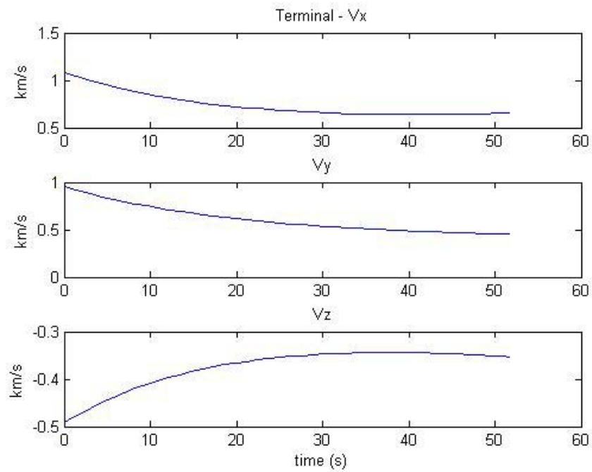
Figure 50: Velocity Breakdown for Terminal Section
