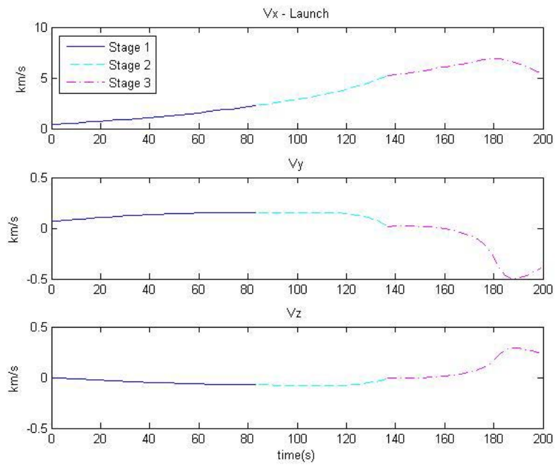
Figure 23: Velocity for Launch Section
