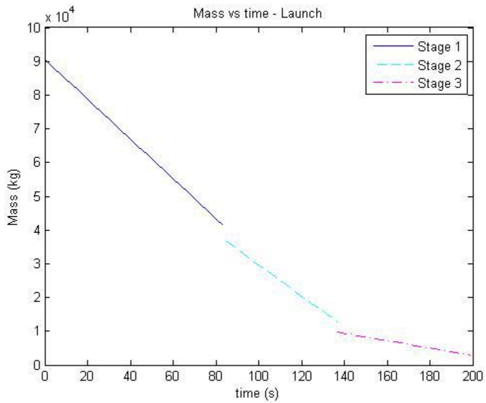
Figure 28: Mass Profile
