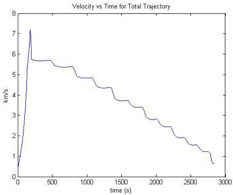
Figure 53: Velocity for Complete Trajectory
