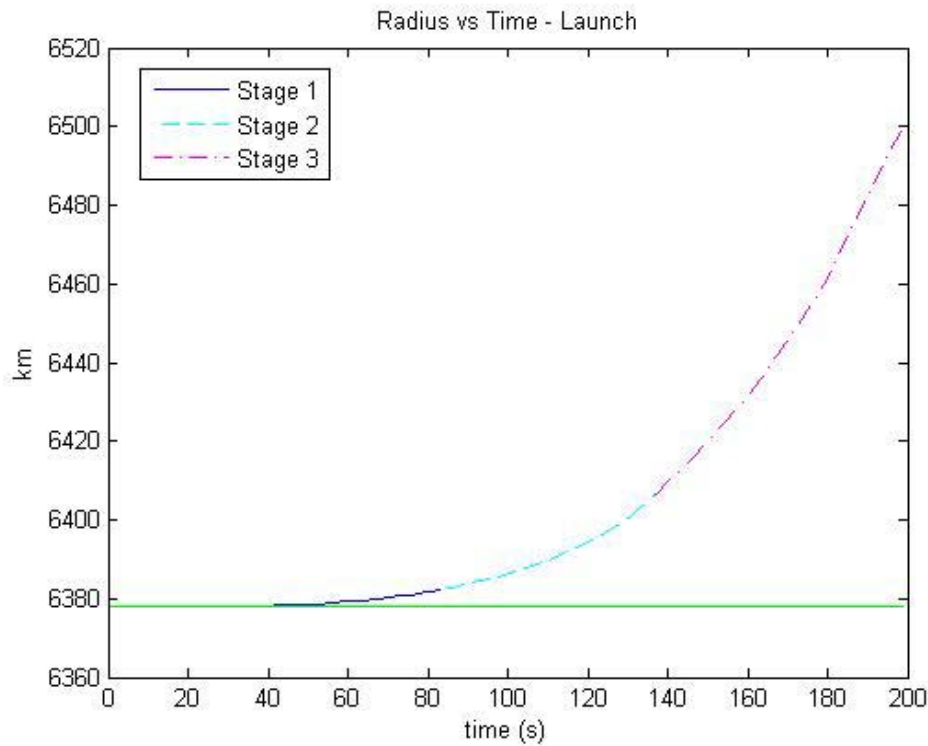
Figure 21: Radius vs. Time for Launch Section
