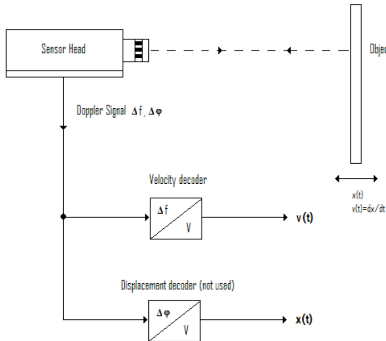
Figure 25. Signals in the Vibrometer (Polytec, 2007)
