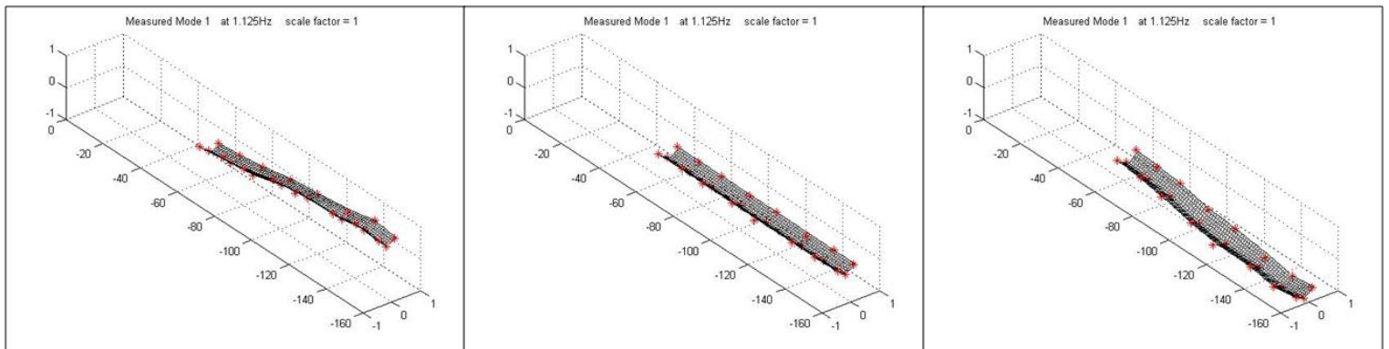
Figure 69. Measured Mode 1 Shape (First Bending about z-axis)
