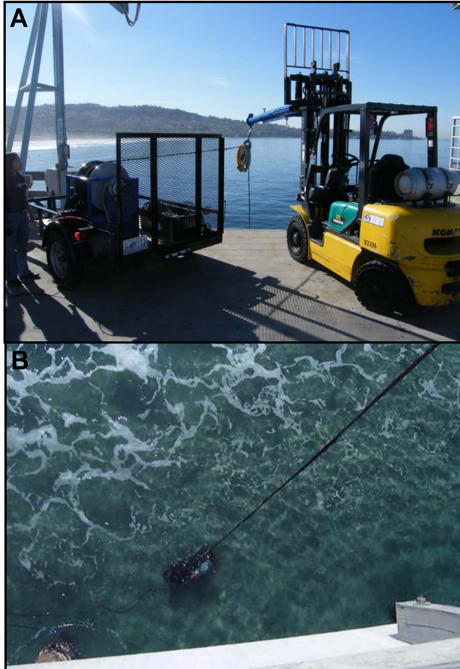
Figure 3. An electric winch and forklift boom with mounted cable block were used as a mobile deployment platform for sampling with the MASCOT sensor package off Scripps Pier, January 2008 (A). Several time series were collected along the length of the pier both in and out of the surf zone (B). Episodic discrete plumes of sediment and bubbles could be observed flowing past the sensor package.
