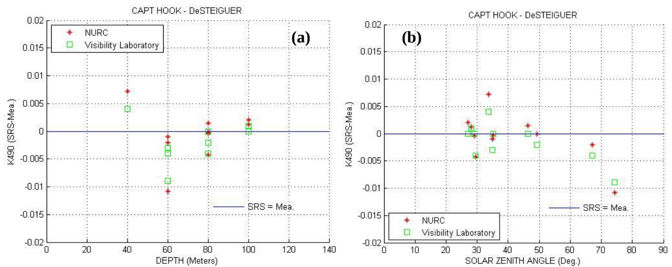
Figure 3: (a) K490 difference error from SRS computations (performed by Visibility Laboratory and NURC) versus depth [meters]. (b) K490 error (estimated – measured) versus solar zenith angle.
