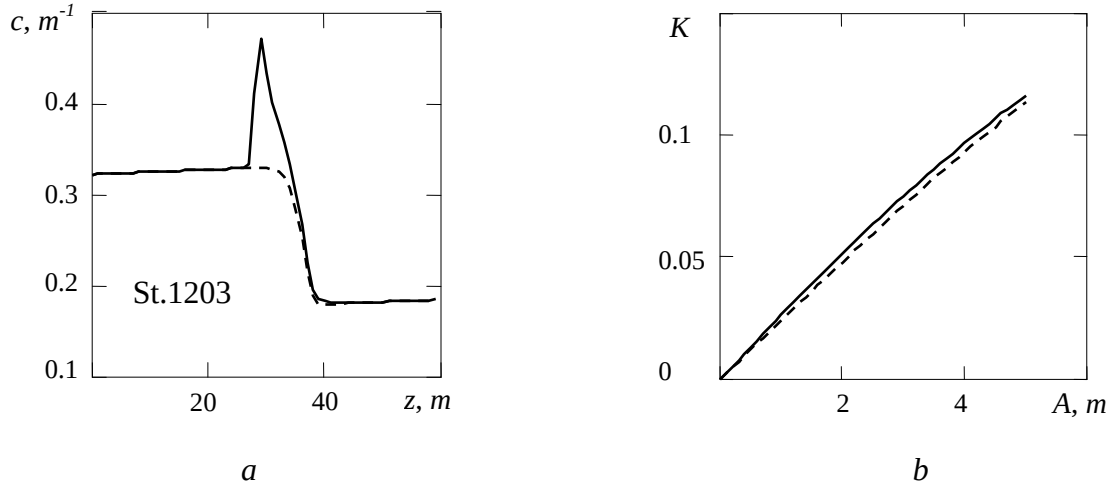
Fig. 1. a) Actual c(z) profile on the station 1203 in the Barents Sea (solid line) and the smoothed profile without the turbid layer (dotted line); b) Computed contrast K of the shadow image of the first IW mode as a function of its amplitude A for the actual (solid line) and smoothed (dotted line) c(z) profiles. The actual pycnocline parameters for station 1203 was used in our computations. Fig. 1b demonstrates a weak dependence of the contrast of IW shadowy image on the thin layer structure in the c(z) profiles.
