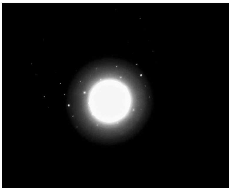
Figure 4. Selected area electron diffraction pattern of the \text{Co}_{0.95}\text{Pd}_{0.05}\text{Te}_{0.05}\text{Sb}_{2.95} alloy after the end of the first discharge/charge cycle.
