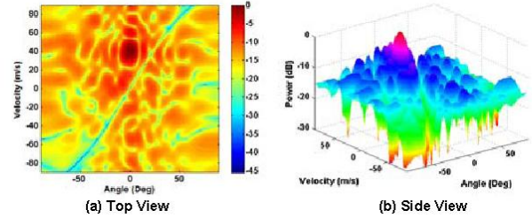
Fig. 6 Average Power Spectrum for 10 sub-bands processed with sample matrix inversion with diagonal loading and subarray/subpulse smoothing ( SMIDLASAPFB ).
