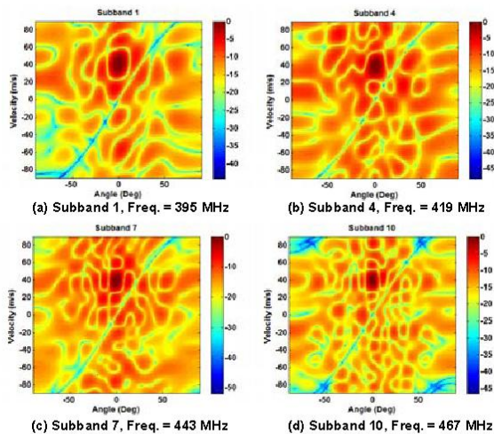
Fig. 5 Angle-Doppler output for different subbands.
