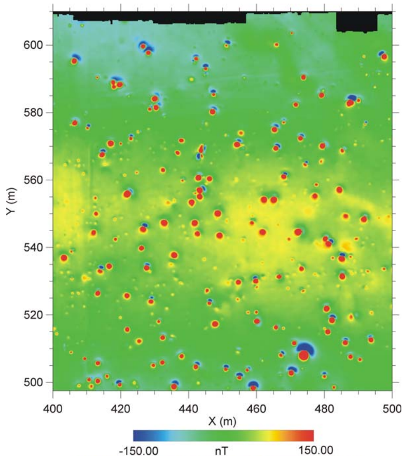
Figure 4. Magnetic anomaly dipole image of Sector A5 on the Buckley Bombing Range.
