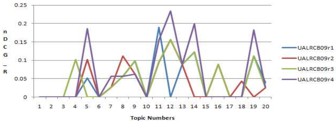
Figure 5: Graph of nDCG_R for all the runs
